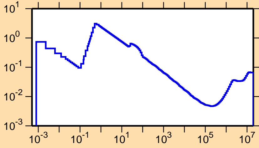
\sigma vs. E for ^{133}\text{Ce}(n,p)
