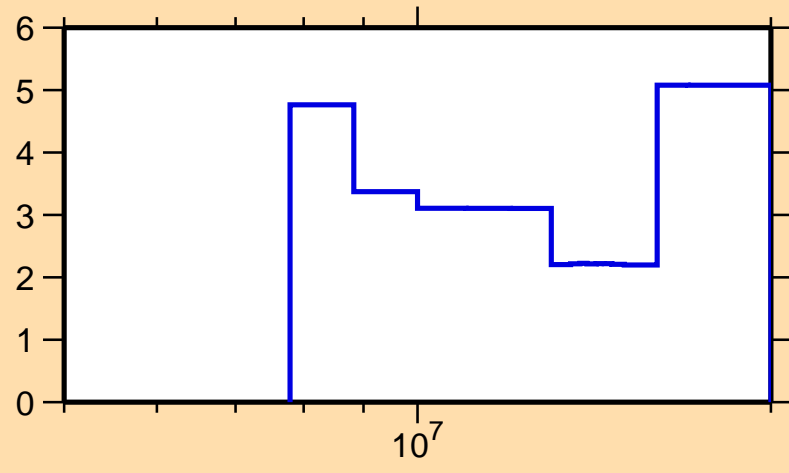
\Delta\sigma/\sigma vs. E for ^{133}\text{Ce}(n,\text{el.})
