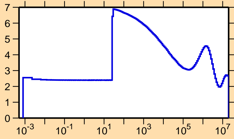
\sigma vs. E for ^{133}\text{Ce}(n,\text{el.})
