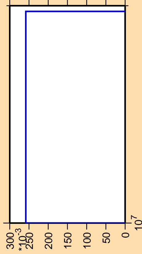
\Delta\sigma/\sigma vs. E for ^{133}\text{Ce} (mt 45)
