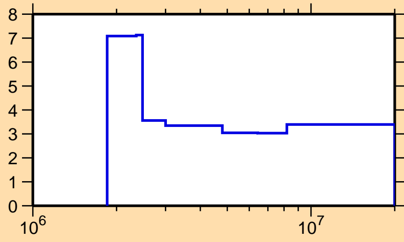
\Delta\sigma/\sigma vs. E for ^{133}\text{Ce}(n,\text{nonel.})
