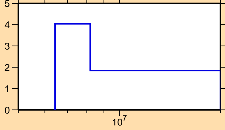
\Delta\sigma/\sigma vs. E for ^{133}\text{Ce}(n,\text{el.})
