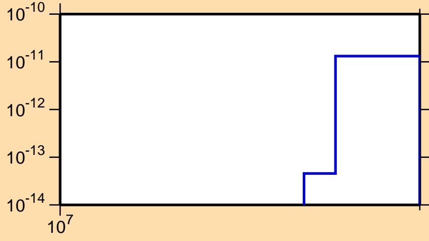
\sigma vs. E for ^{134}\text{Ce} (mt 45)
