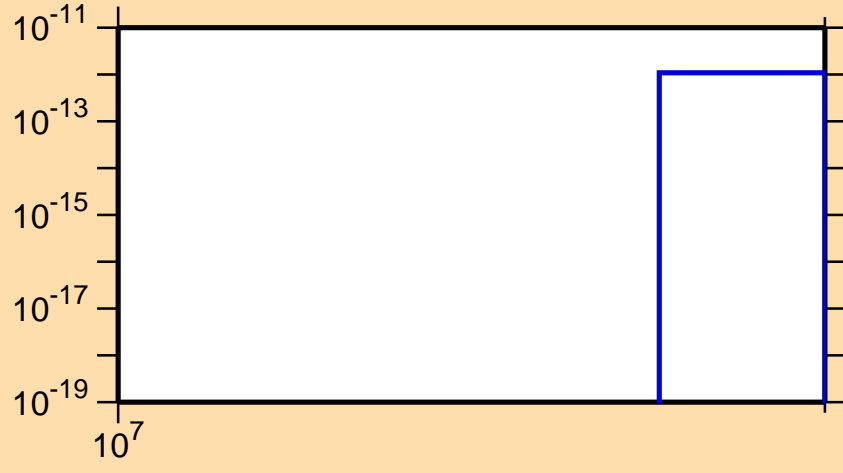
\sigma vs. E for ^{134}\text{Ce}(n,nt)
