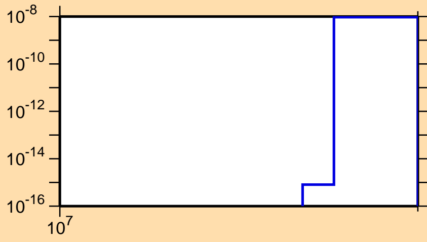
\sigma vs. E for ^{134}\text{Ce}(n,2np)
