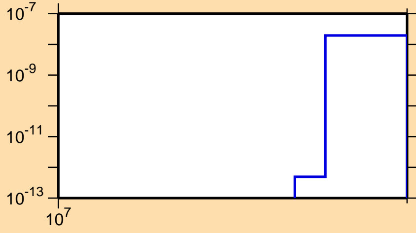
\sigma vs. E for ^{134}\text{Ce}(n,\text{nd})
