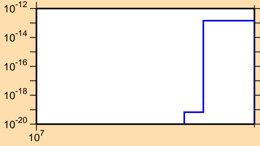
\sigma vs. E for ^{134}\text{Ce}(n,\text{pt})
