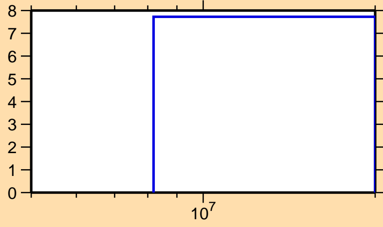
\Delta\sigma/\sigma vs. E for ^{134}\text{Ce}(n,\text{inel.})
