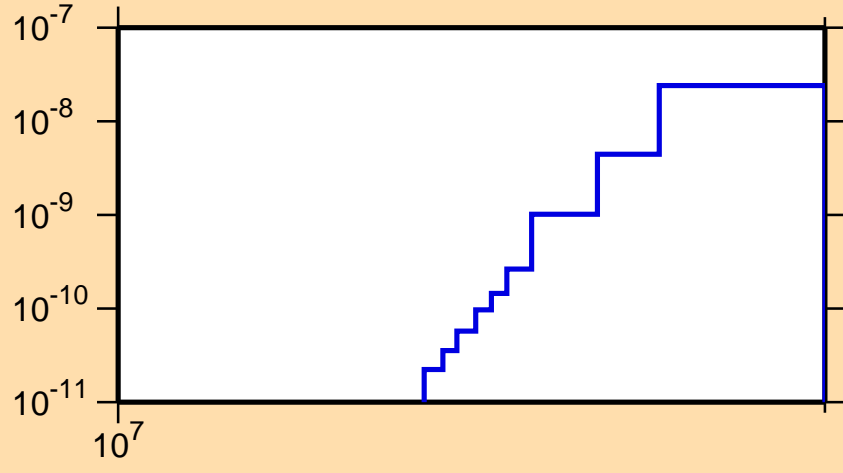
\sigma vs. E for ^{136}\text{Ce}(n,p\alpha)
