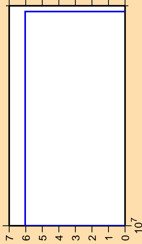
\Delta\sigma/\sigma vs. E for ^{136}\text{Ce}(n,2np)
