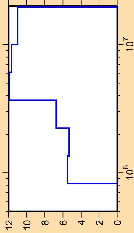
\Delta\sigma/\sigma vs. E for ^{136}\text{Ce}(n,n_2)
