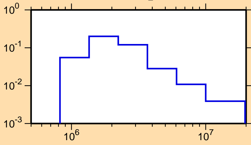
\sigma vs. E for ^{136}\text{Ce}(n,n_2)
