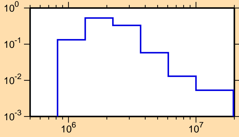
\sigma vs. E for ^{136}\text{Ce}(n,n_3)
