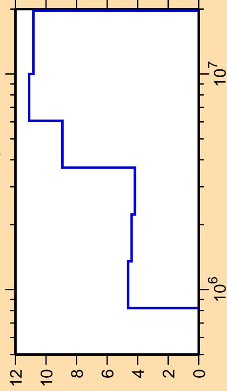
\Delta\sigma/\sigma vs. E for ^{136}\text{Ce}(n,n_3)
