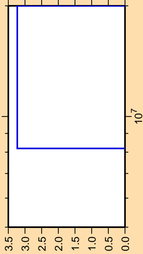
\Delta\sigma/\sigma vs. E for ^{136}\text{Ce}(n,pd)
