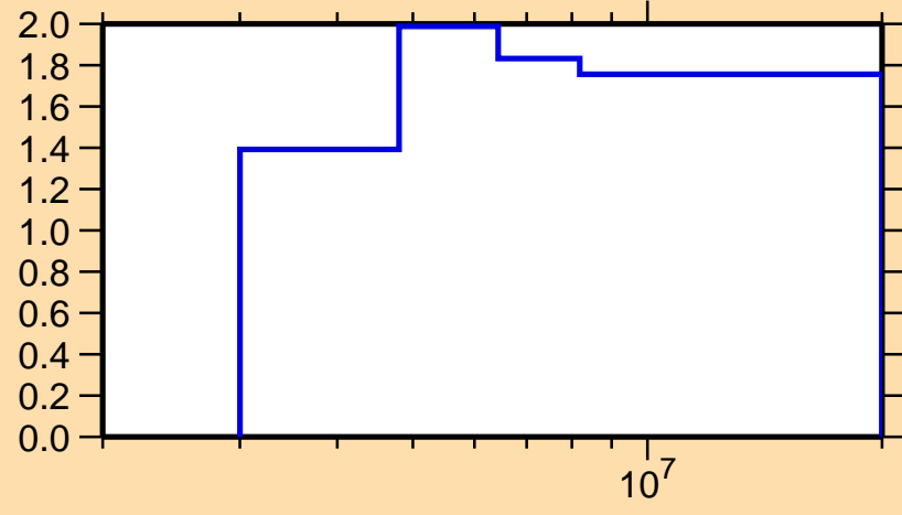
\Delta\sigma/\sigma vs. E for ^{136}\text{Ce}(n,n\text{onel.})
