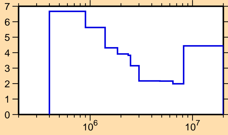
\Delta\sigma/\sigma vs. E for ^{136}\text{Ce}(n,\text{inel.})
