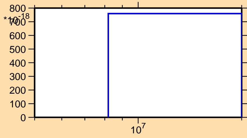
\sigma vs. E for ^{136}\text{Ce}(\text{mt } 45)
