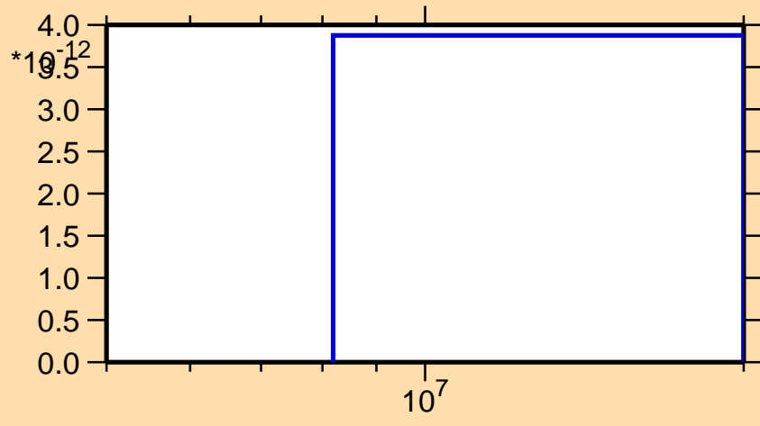
\sigma vs. E for ^{136}\text{Ce}(n,pd)
