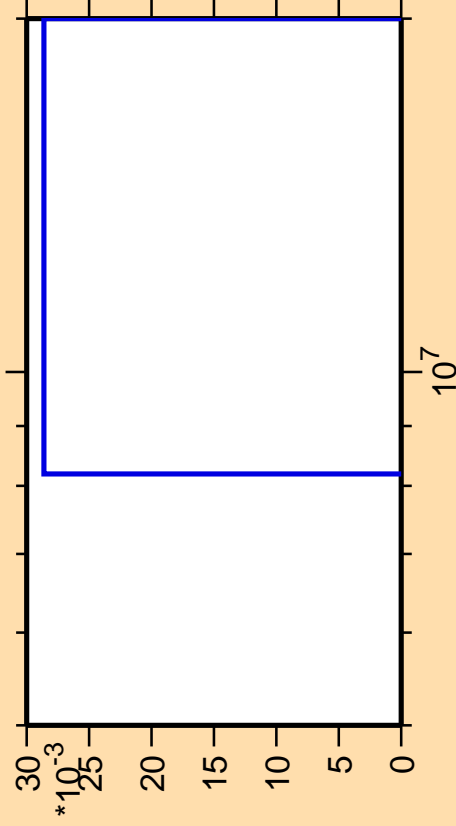
\Delta\sigma/\sigma vs. E for ^{136}\text{Ce}(n,nt)
