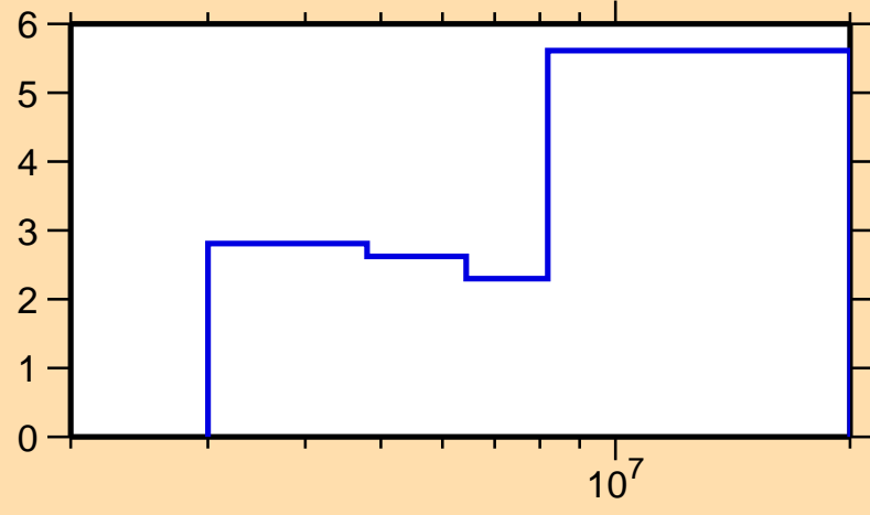
\Delta\sigma/\sigma vs. E for ^{136}\text{Ce}(n,n\text{cont.})
