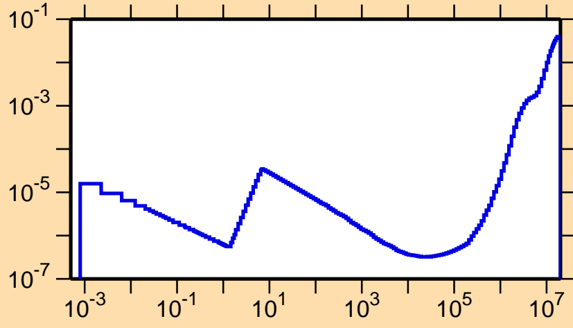
\sigma vs. E for ^{137}\text{Ce}(n,p)
