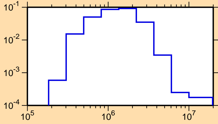
\sigma vs. E for ^{137}\text{Ce}(n,n_2)
