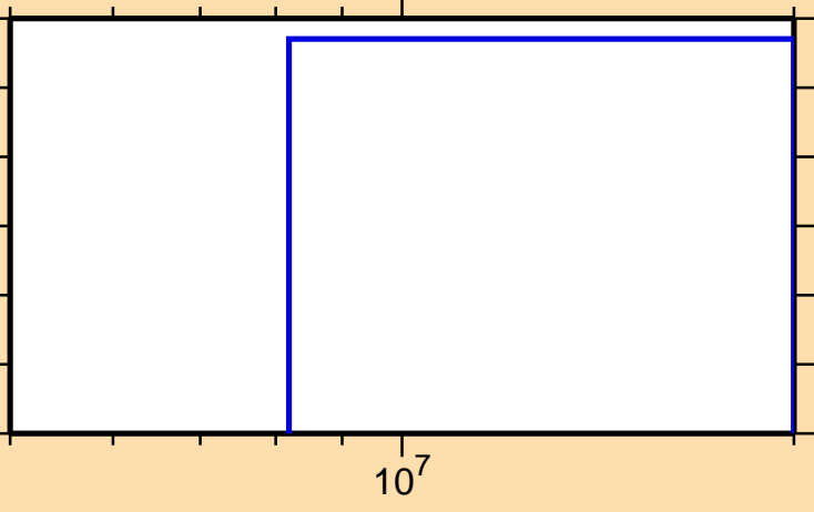
\sigma vs. E for ^{137}\text{Ce}(n,\text{pd})
