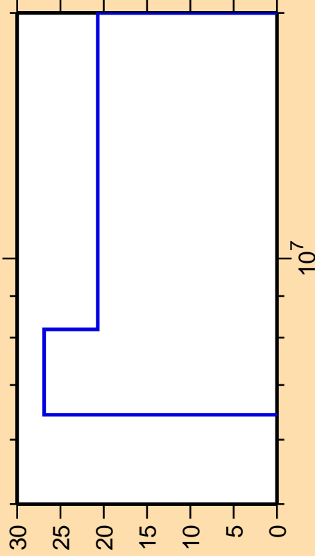
\Delta\sigma/\sigma vs. E for ^{137}\text{Ce}(n,p)
