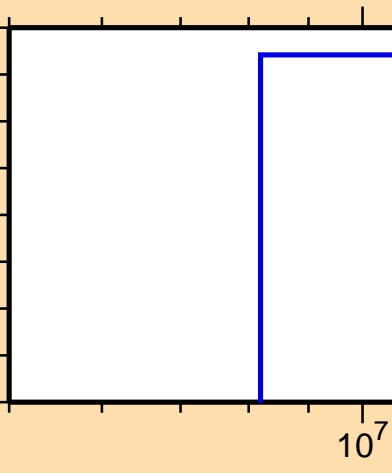
\sigma vs. E for ^{137}\text{Ce}(n,np)
