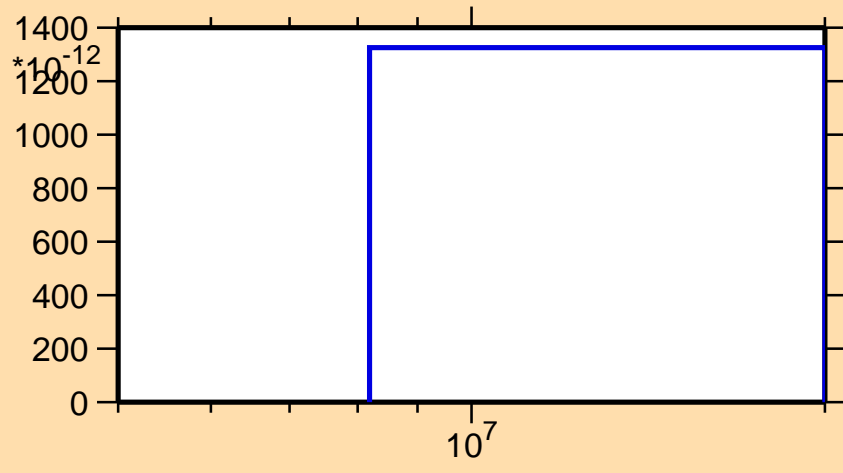
\sigma vs. E for ^{137}\text{Ce}(n,p\alpha)
