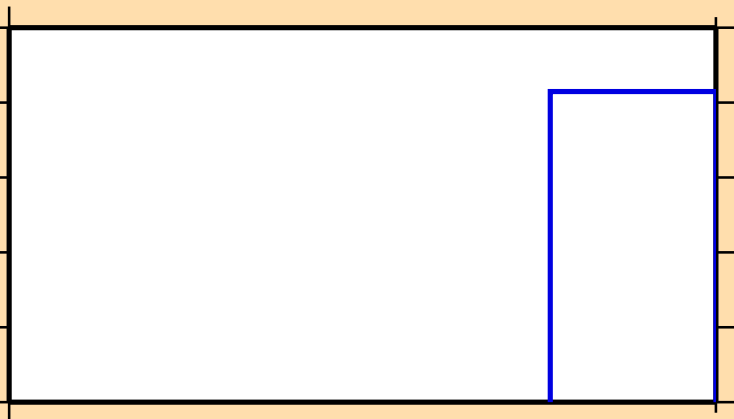
\sigma vs. E for ^{137}\text{Ce}(n,3n)
