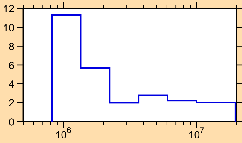
\Delta\sigma/\sigma vs. E for ^{137}\text{Ce}(n,\text{nonel.})
