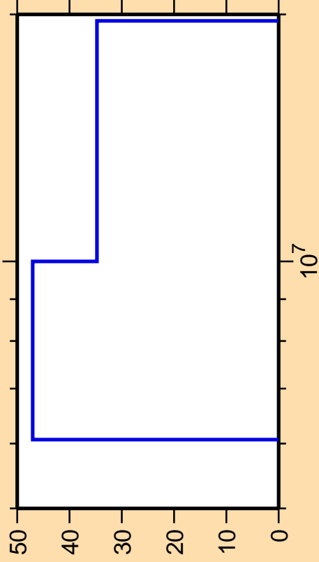
\Delta\sigma/\sigma vs. E for ^{137}\text{Ce}(n,np)
