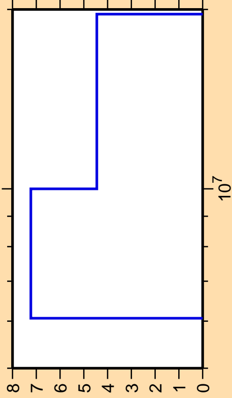
\Delta\sigma/\sigma vs. E for ^{137}\text{Ce}(n,2n)
