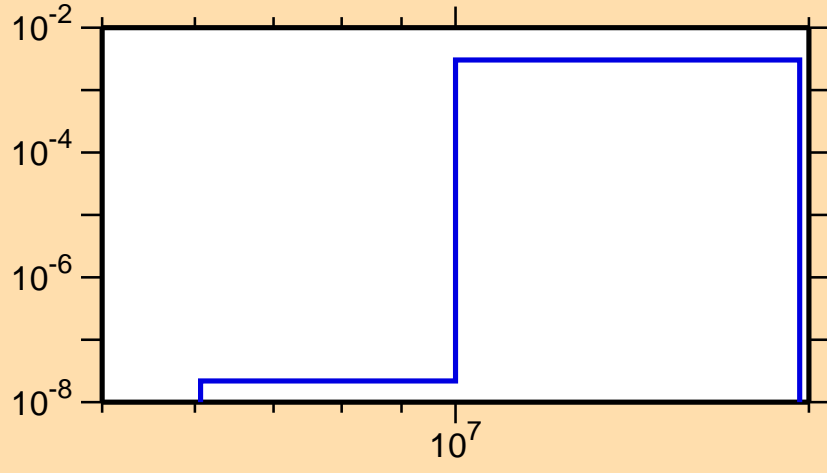
\sigma vs. E for ^{137}\text{Ce}(n,np)
