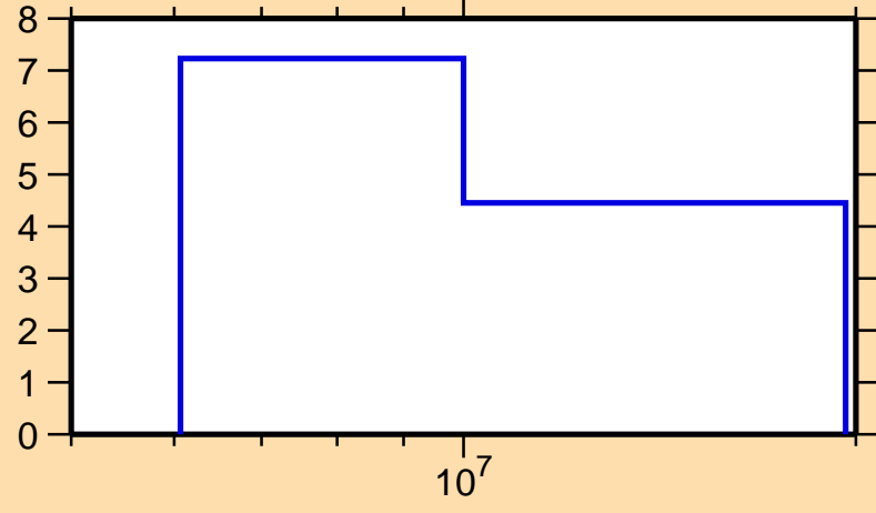
\Delta\sigma/\sigma vs. E for ^{137}\text{Ce}(n,2n)
