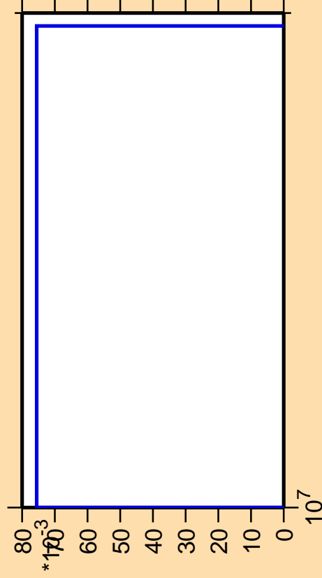
\Delta\sigma/\sigma vs. E for ^{137}\text{Ce}(n,pd)
