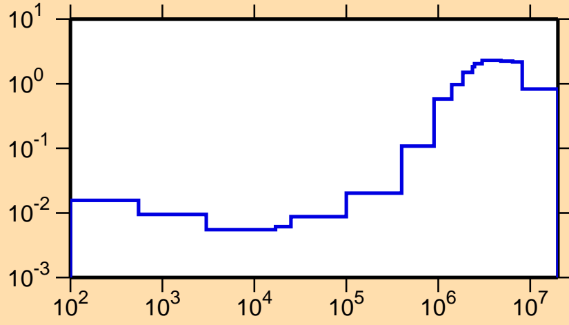
\sigma vs. E for ^{137}\text{Ce}(n,\text{inel.})
