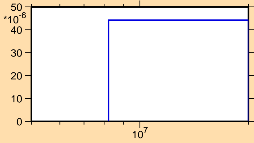
\sigma vs. E for ^{137}\text{Ce}(n,t)
