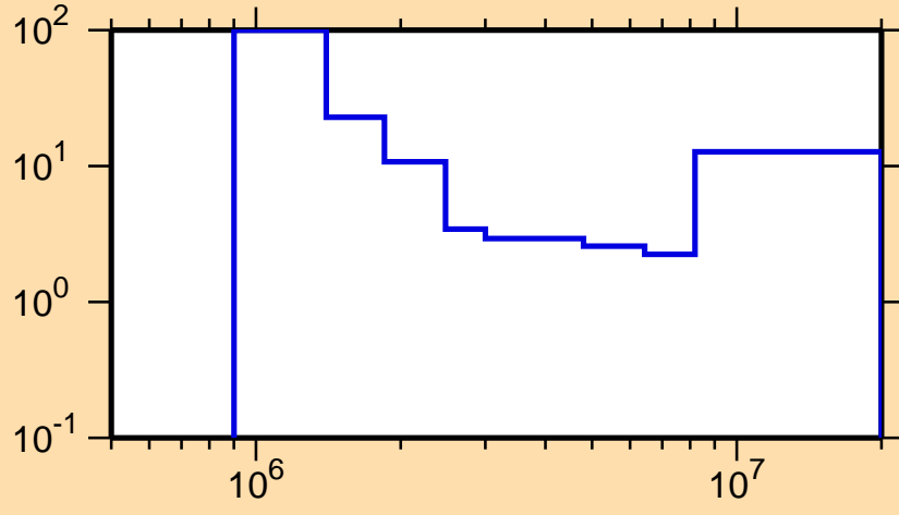
\Delta\sigma/\sigma vs. E for ^{137}\text{Ce}(n,n\text{cont.})
