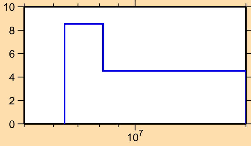
\Delta\sigma/\sigma vs. E for ^{137}\text{Ce}(n,2n)
