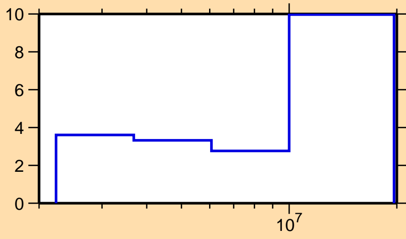
\Delta\sigma/\sigma vs. E for ^{138}\text{Ce}(n,n\text{cont.})
