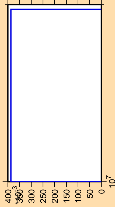
\Delta\sigma/\sigma vs. E for ^{138}\text{Ce}(n,2np)
