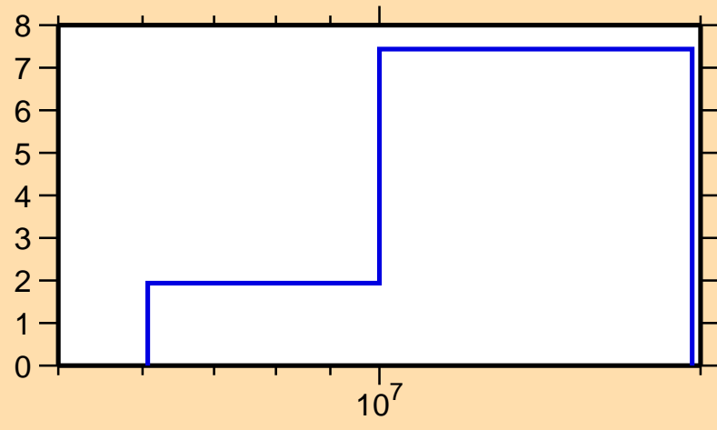
\Delta\sigma/\sigma vs. E for ^{138}\text{Ce}(n,\text{inel.})
