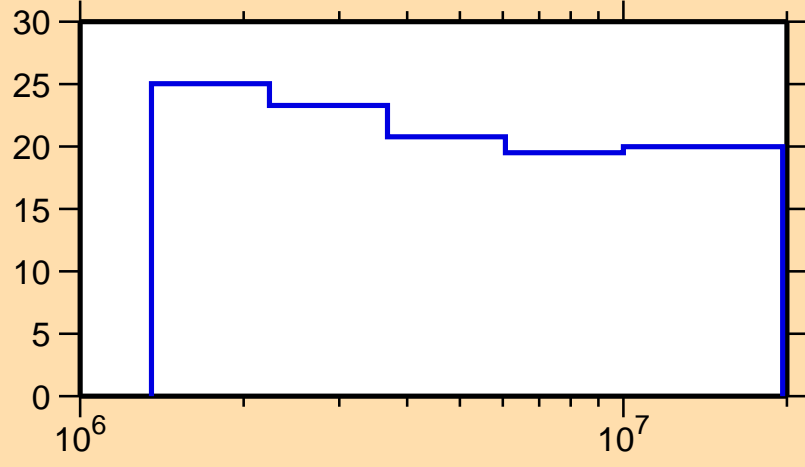
\Delta\sigma/\sigma vs. E for ^{138}\text{Ce}(n,p)
