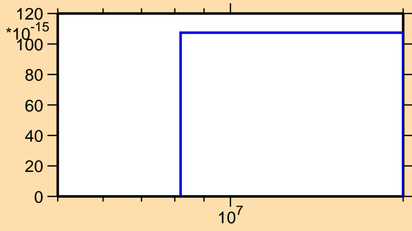
\sigma vs. E for ^{138}\text{Ce}(n,\text{pd})
