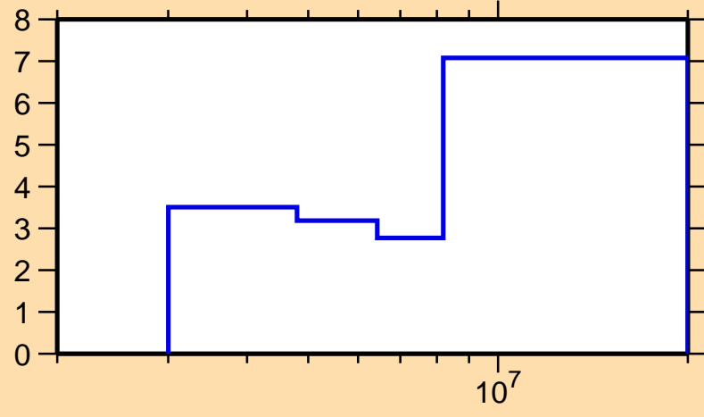
\Delta\sigma/\sigma vs. E for ^{138}\text{Ce}(n,n\text{cont.})
