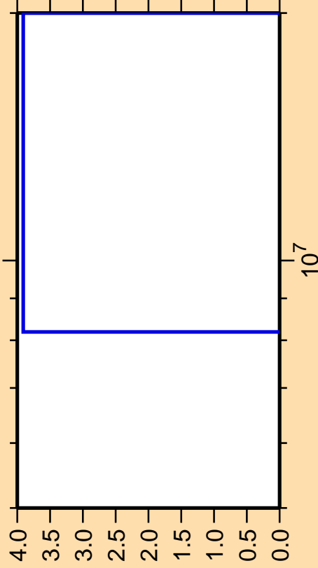
\Delta\sigma/\sigma vs. E for ^{138}\text{Ce}(n,2n)
