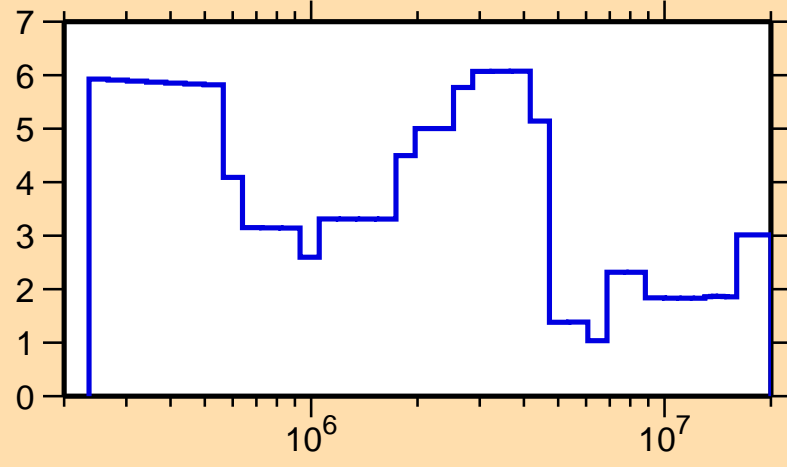
\Delta\sigma/\sigma vs. E for ^{139}\text{Ce}(n,\text{el.})
