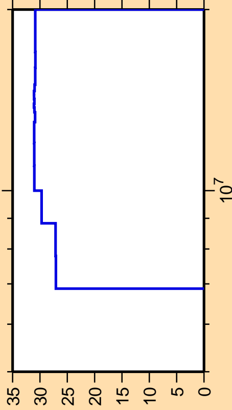
\Delta\sigma/\sigma vs. E for ^{139}\text{Ce}(n,\gamma)
