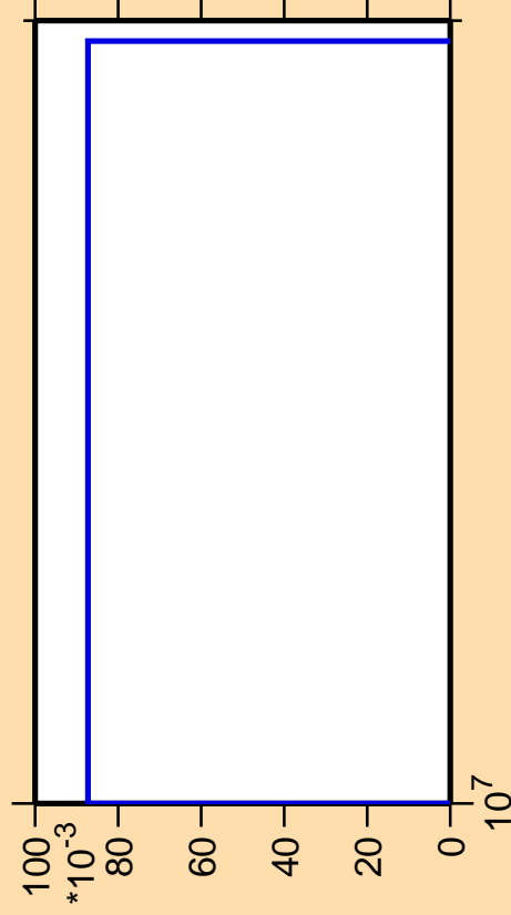
\Delta\sigma/\sigma vs. E for ^{139}\text{Ce}(n,nt)
