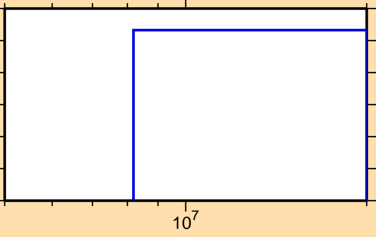
\sigma vs. E for ^{139}\text{Ce}(n,\text{nd})
