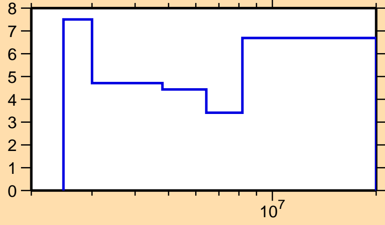
\Delta\sigma/\sigma vs. E for ^{139}\text{Ce}(n,n\text{cont.})
