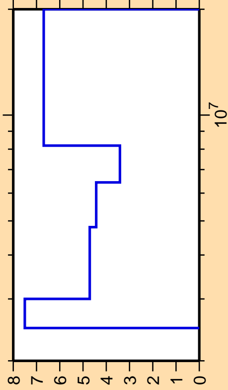
\Delta\sigma/\sigma vs. E for ^{139}\text{Ce}(n,n\text{cont.})
