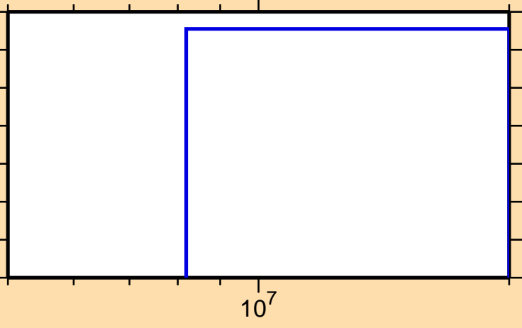
\sigma vs. E for ^{139}\text{Ce}(n,t)
