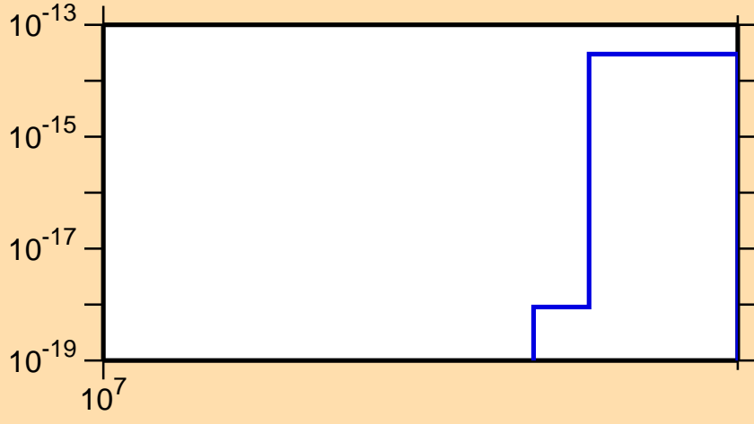
\sigma vs. E for ^{139}\text{Ce} (mt 34)
