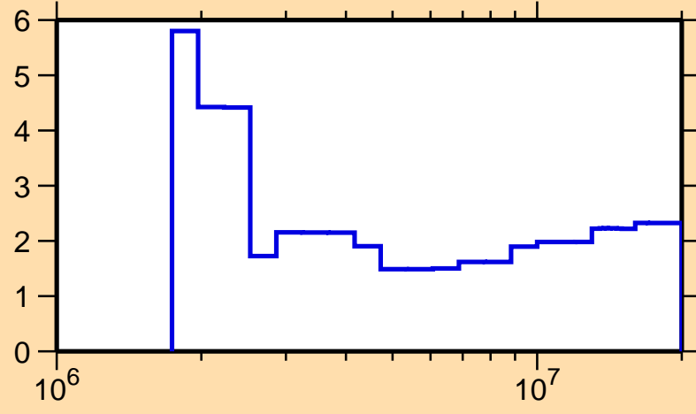
\Delta\sigma/\sigma vs. E for ^{139}\text{Ce}(n,n\text{onel.})
