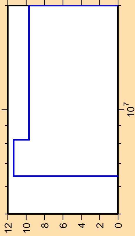
\Delta\sigma/\sigma vs. E for ^{139}\text{Ce}(n,p)
