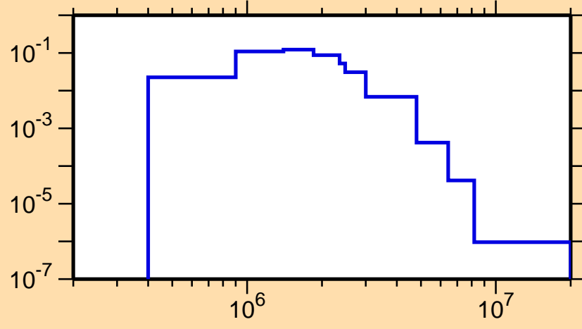
\sigma vs. E for ^{139}\text{Ce}(n,n_4)
