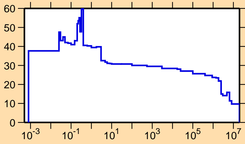
\Delta\sigma/\sigma vs. E for ^{139}\text{Ce}(n,p)
