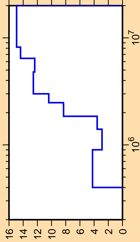
\Delta\sigma/\sigma vs. E for ^{139}\text{Ce}(n,n_4)
