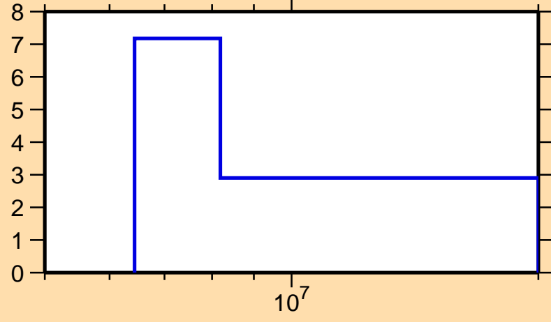
\Delta\sigma/\sigma vs. E for ^{139}\text{Ce}(n,2n)
