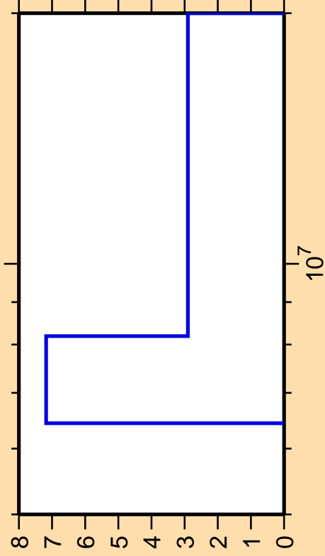
\Delta\sigma/\sigma vs. E for ^{139}\text{Ce}(n,2n)
