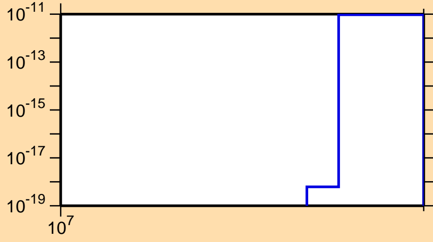
\sigma vs. E for ^{140}\text{Ce}(n,nt)
