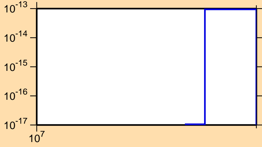
\sigma vs. E for ^{140}\text{Ce}(n,\text{pd})
