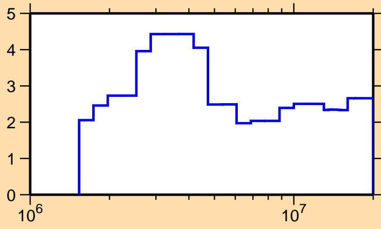
\Delta\sigma/\sigma vs. E for ^{140}\text{Ce}(n,\text{el.})
