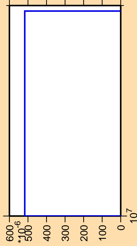
\Delta\sigma/\sigma vs. E for ^{140}\text{Ce}(n,pd)
