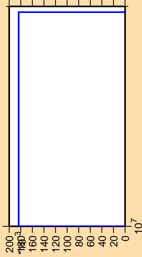
\Delta\sigma/\sigma vs. E for ^{140}\text{Ce}(n,p\alpha)
