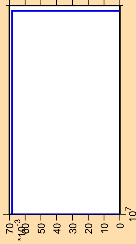
\Delta\sigma/\sigma vs. E for ^{140}\text{Ce}(n,nt)
