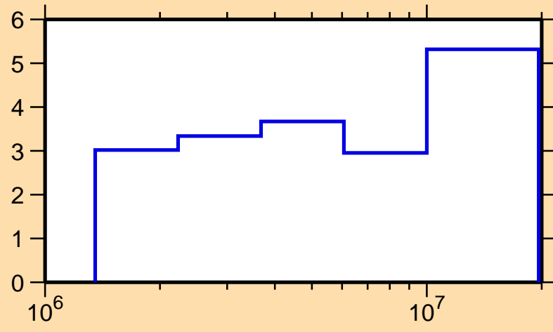
\Delta\sigma/\sigma vs. E for ^{140}\text{Ce}(n,\text{inel.})
