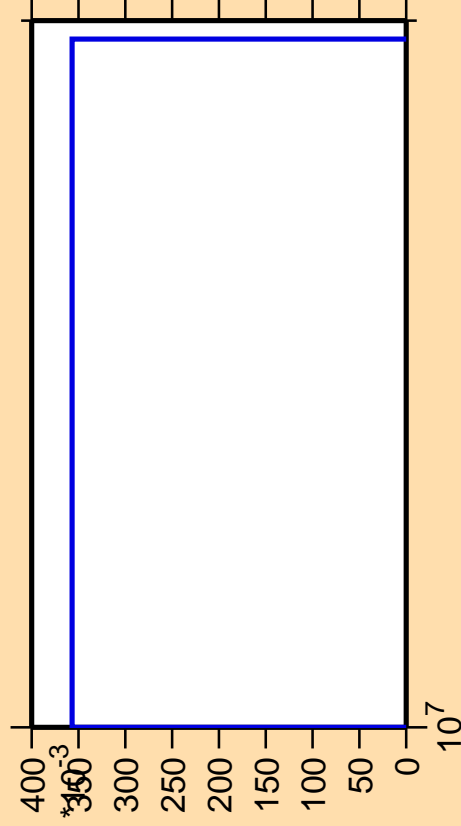
\Delta\sigma/\sigma vs. E for ^{140}\text{Ce}(n,2np)
