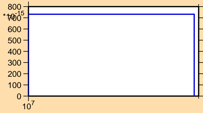
\sigma vs. E for ^{140}\text{Ce}(n,2np)
