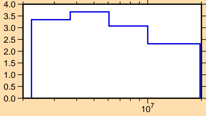
\Delta\sigma/\sigma vs. E for ^{140}\text{Ce}(n,n\text{onel.})
