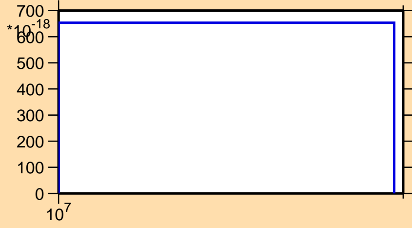
\sigma vs. E for ^{140}\text{Ce}(n,pd)
