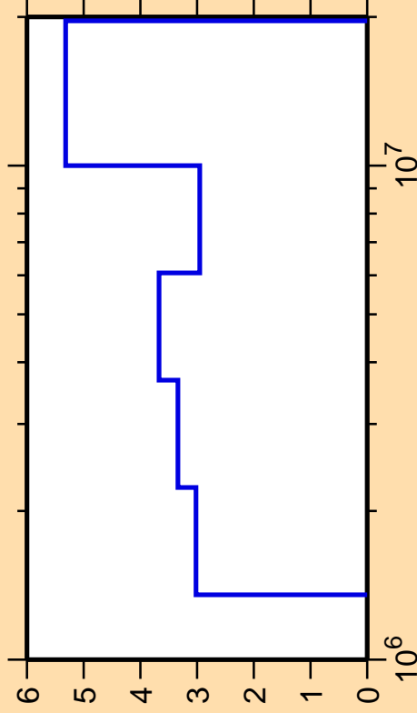
\Delta\sigma/\sigma vs. E for ^{140}\text{Ce}(n,\text{inel.})
