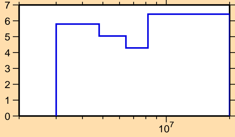
\Delta\sigma/\sigma vs. E for ^{140}\text{Ce}(n,n\text{cont.})
