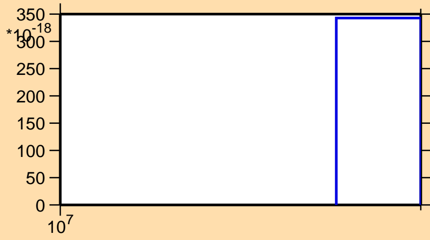
\sigma vs. E for ^{143}\text{Ce} (mt 11)
