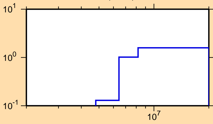
\sigma vs. E for ^{143}\text{Ce}(n,2n)
