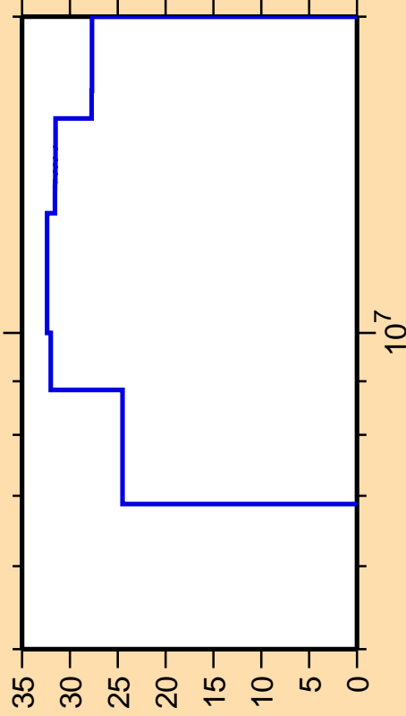
\Delta\sigma/\sigma vs. E for ^{144}\text{Ce}(n,p)
