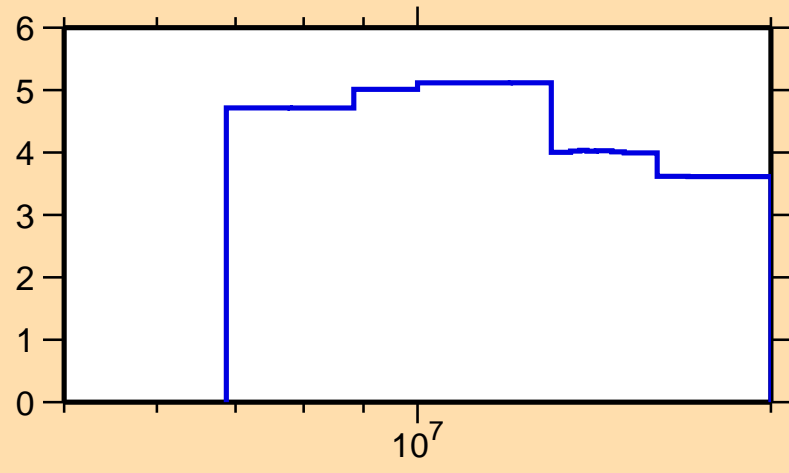
\Delta\sigma/\sigma vs. E for ^{144}\text{Ce}(n,\text{nonel.})
