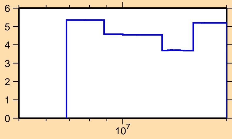
\Delta\sigma/\sigma vs. E for ^{144}\text{Ce}(n,\text{el.})
