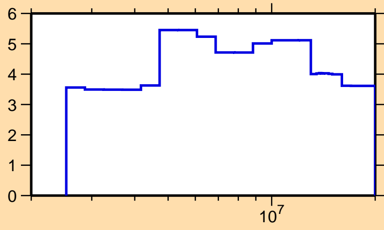
\Delta\sigma/\sigma vs. E for ^{144}\text{Ce}(n,n\text{onel.})
