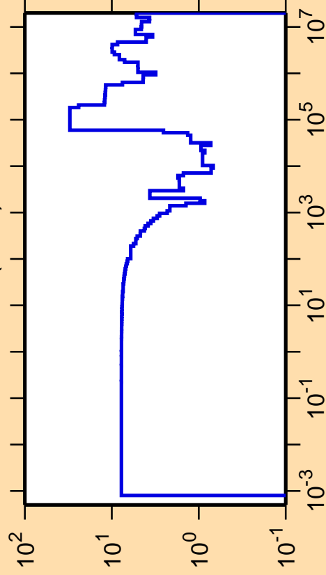
\Delta\sigma/\sigma vs. E for ^{144}\text{Ce}(n,\text{el.})
