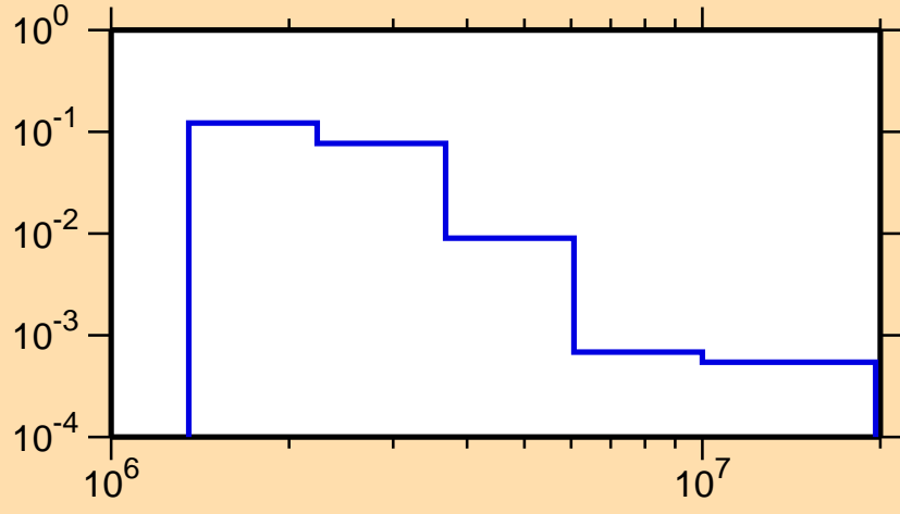
\sigma vs. E for ^{144}\text{Ce}(n,n_4)
