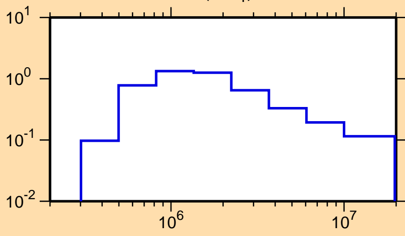
\sigma vs. E for ^{144}\text{Ce}(n,n_1)
