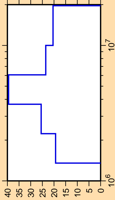
\Delta\sigma/\sigma vs. E for ^{144}\text{Ce}(n,n_4)
