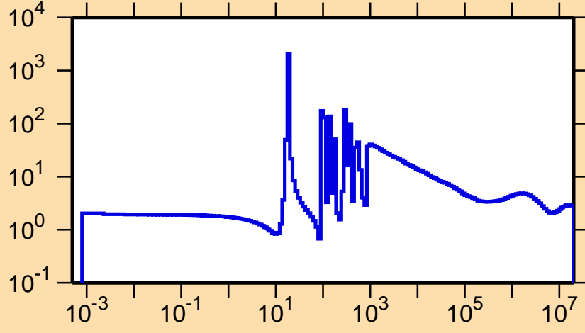
\sigma vs. E for ^{145}\text{Ce}(n,\text{el.})
