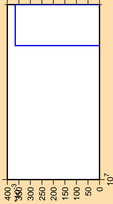
\Delta\sigma/\sigma vs. E for ^{145}\text{Ce}(n,p\alpha)
