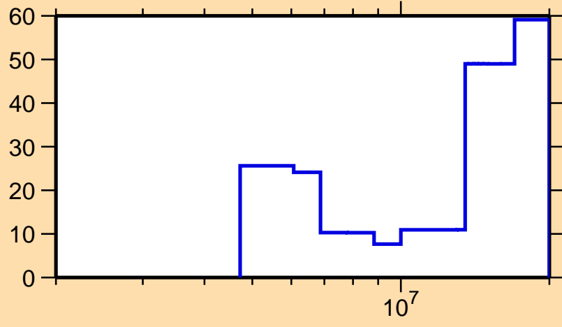
\Delta\sigma/\sigma vs. E for ^{145}\text{Ce}(n,2n)
