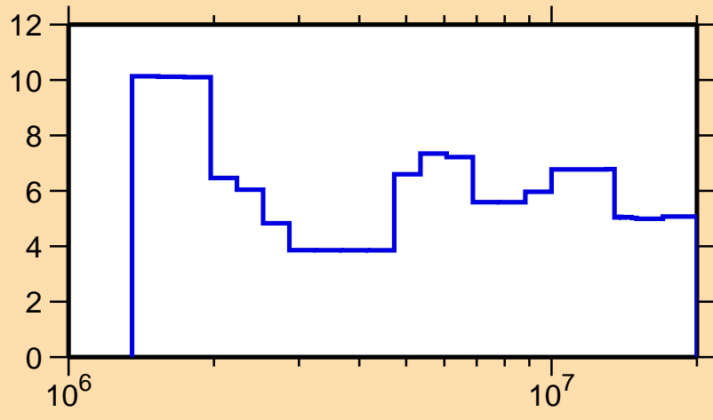
\Delta\sigma/\sigma vs. E for ^{145}\text{Ce}(n,\text{nonel.})
