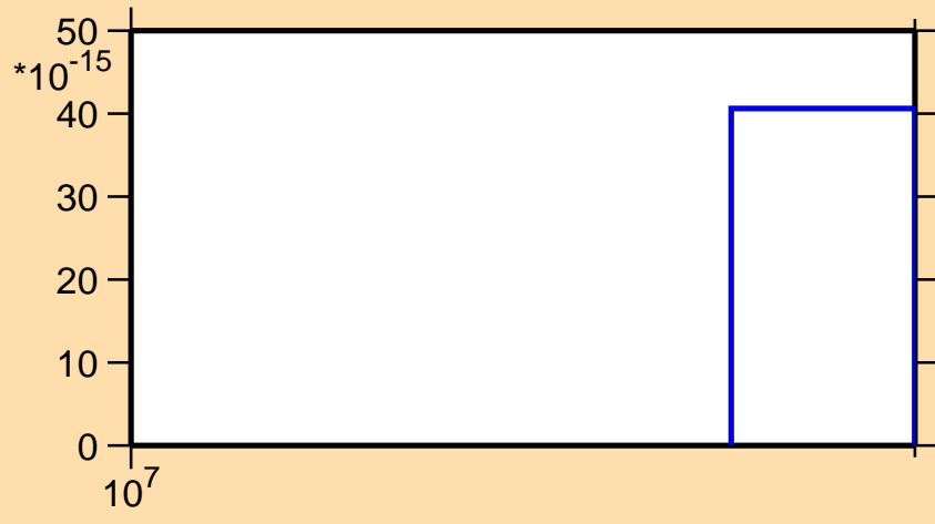
\sigma vs. E for ^{145}\text{Ce}(n,p\alpha)
