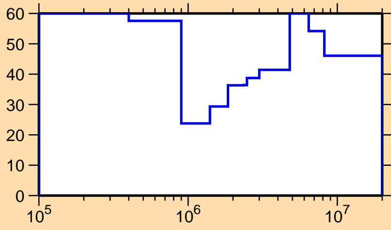
\Delta\sigma/\sigma vs. E for ^{146}\text{Ce}(n,n_1)
