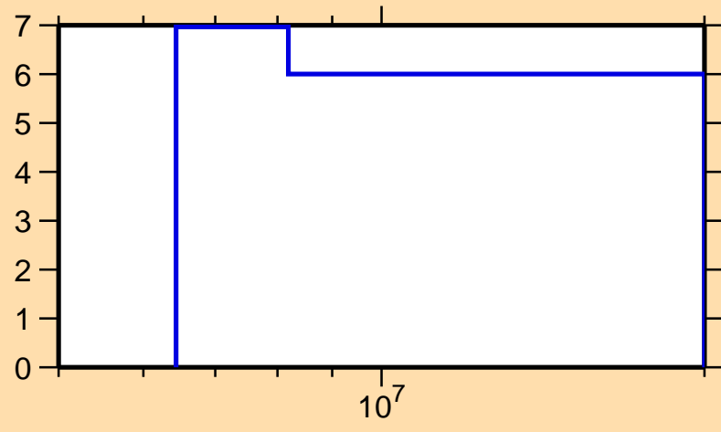
\Delta\sigma/\sigma vs. E for ^{146}\text{Ce}(n,\text{nonel.})
