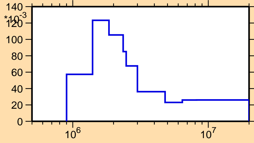
\sigma vs. E for ^{146}\text{Ce}(n,n_4)
