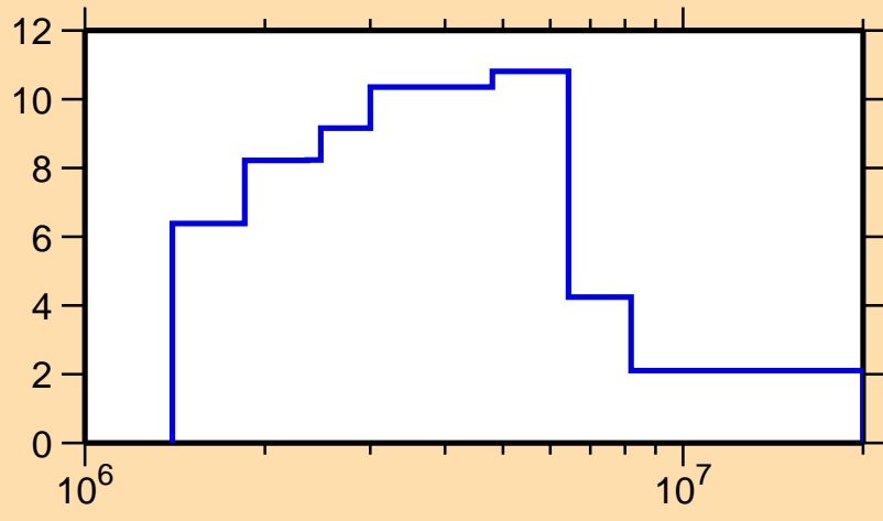
\Delta\sigma/\sigma vs. E for ^{146}\text{Ce}(n,\text{tot.})
