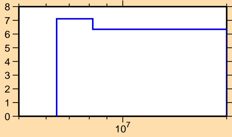
\Delta\sigma/\sigma vs. E for ^{146}\text{Ce}(n,\text{el.})
