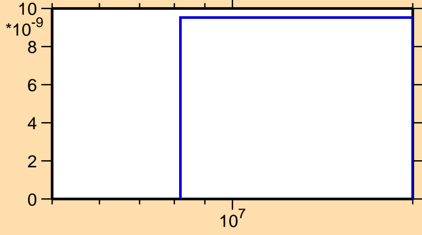
\sigma vs. E for ^{146}\text{Ce}(n,nt)
