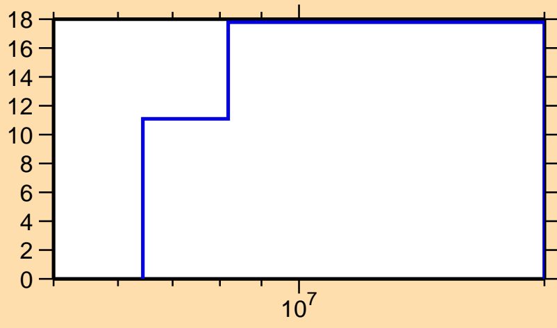
\Delta\sigma/\sigma vs. E for ^{146}\text{Ce}(n,2n)
