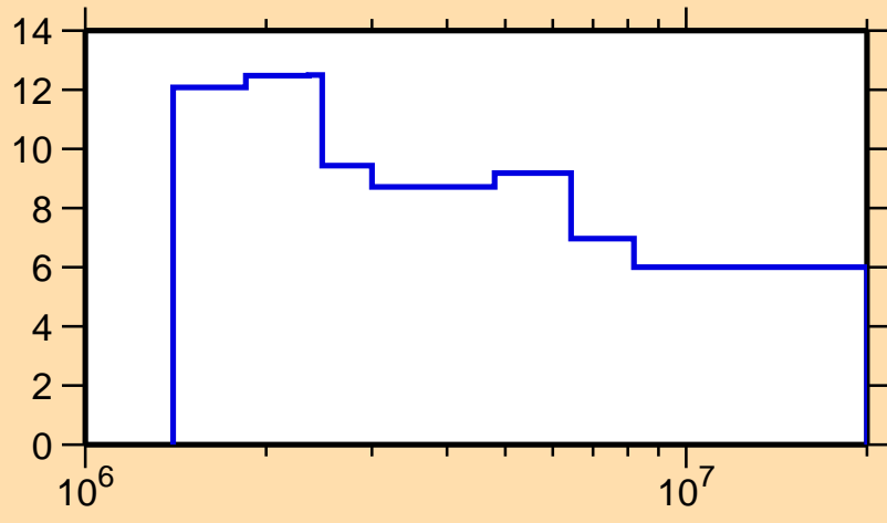
\Delta\sigma/\sigma vs. E for ^{146}\text{Ce}(n,\text{nonel.})
