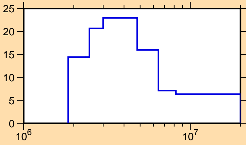
\Delta\sigma/\sigma vs. E for ^{146}\text{Ce}(n,\text{el.})
