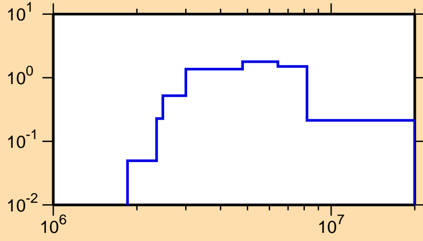
\sigma vs. E for ^{146}\text{Ce}(n,n\text{cont.})
