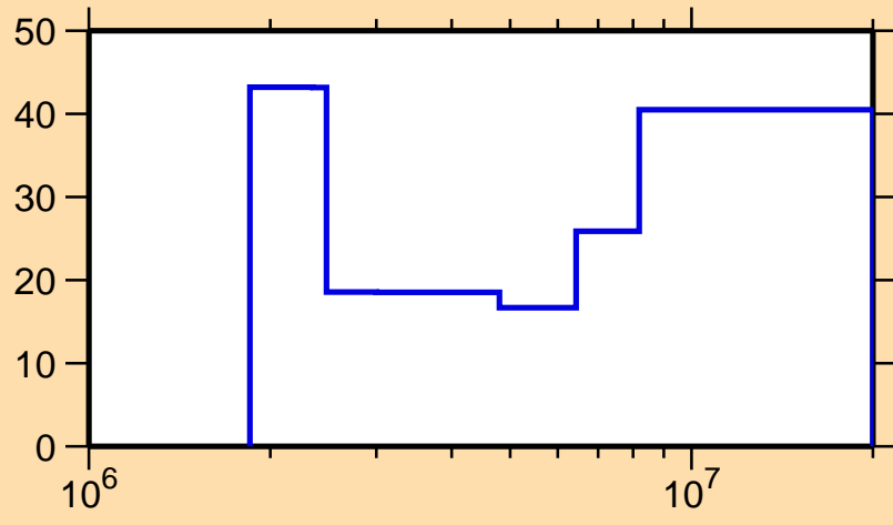
\Delta\sigma/\sigma vs. E for ^{146}\text{Ce}(n,n\text{cont.})
