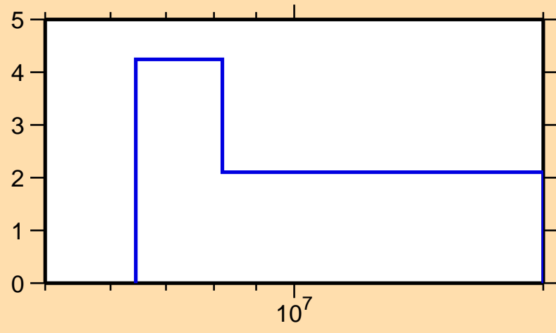
\Delta\sigma/\sigma vs. E for ^{146}\text{Ce}(n,\text{tot.})
