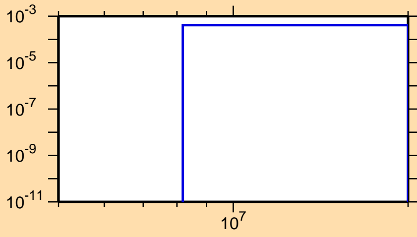
\sigma vs. E for ^{146}\text{Ce}(n,p)
