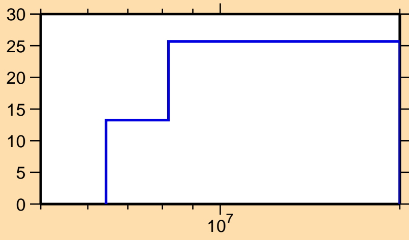
\Delta\sigma/\sigma vs. E for ^{146}\text{Ce}(n,\text{inel.})
