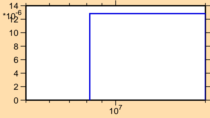
\sigma vs. E for ^{146}\text{Ce}(n,np)
