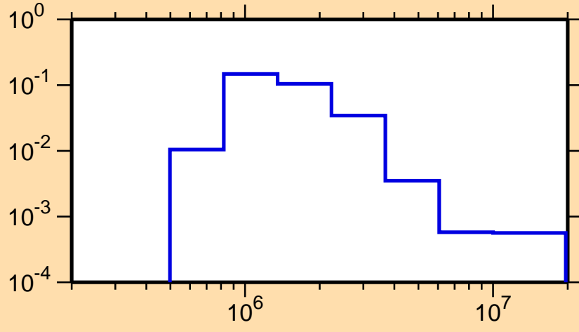
\sigma vs. E for ^{148}\text{Ce}(n,n_3)
