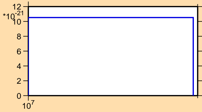
\sigma vs. E for ^{148}\text{Ce} (mt 11)
