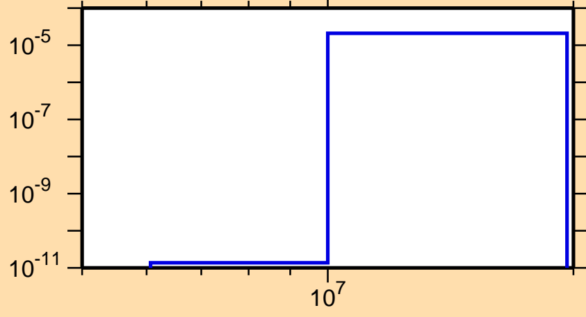
\sigma vs. E for ^{148}\text{Ce}(n,n\alpha)
