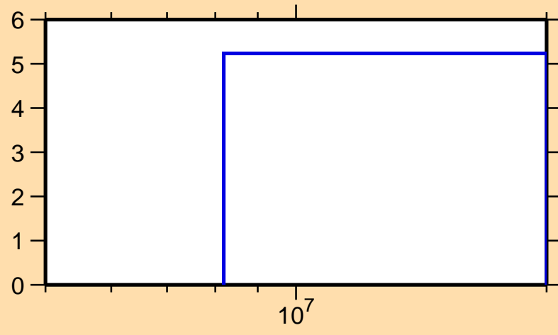
\Delta\sigma/\sigma vs. E for ^{148}\text{Ce}(n,\text{tot.})
