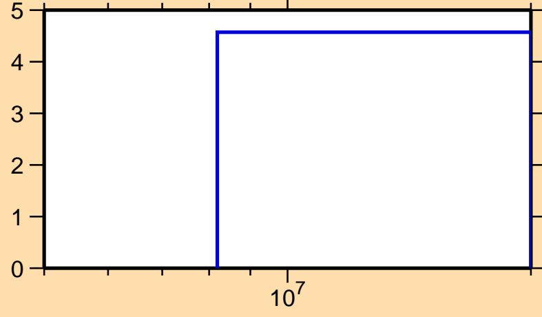
\Delta\sigma/\sigma vs. E for ^{148}\text{Ce}(n,\text{el.})
