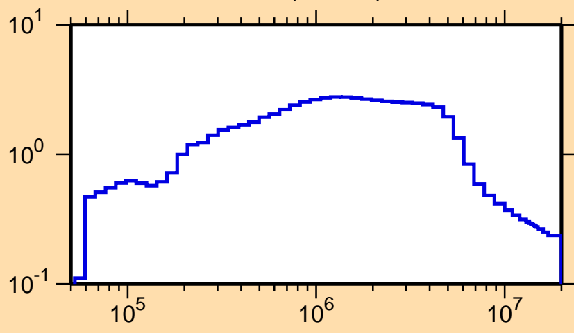
\sigma vs. E for ^{149}\text{Ce}(n,\text{inel.})
