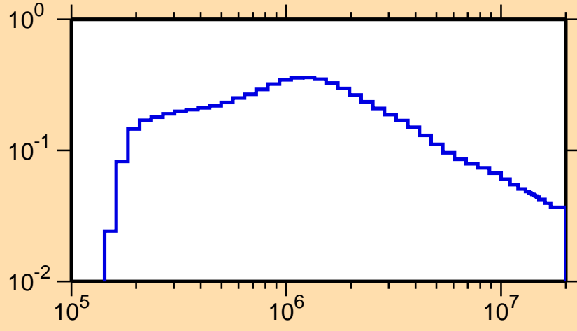
\sigma vs. E for ^{149}\text{Ce}(n,n_3)
