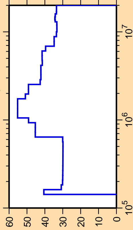
\Delta\sigma/\sigma vs. E for ^{149}\text{Ce}(n,n_3)
