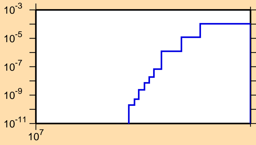
\sigma vs. E for ^{149}\text{Ce}(n,np)
