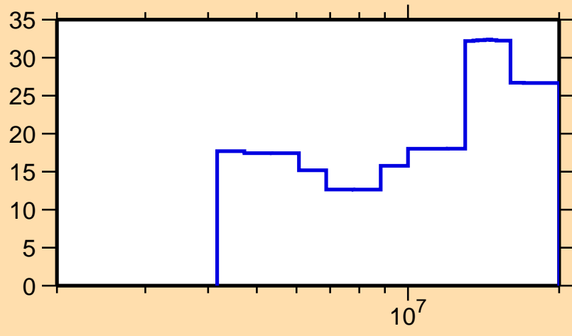
\Delta\sigma/\sigma vs. E for ^{149}\text{Ce}(n,2n)
