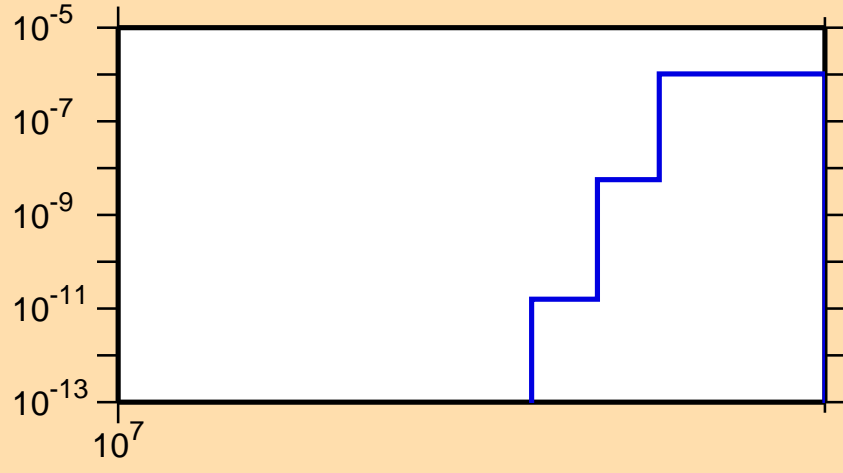
\sigma vs. E for ^{149}\text{Ce}(n,nt)
