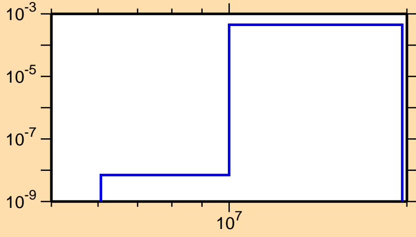
\sigma vs. E for ^{149}\text{Ce}(n,p)
