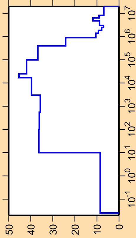
\Delta\sigma/\sigma vs. E for ^{149}\text{Ce}(n,\text{nonel.})
