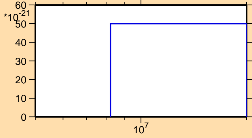
\sigma vs. E for ^{149}\text{Ce}(\text{mt } 11)
