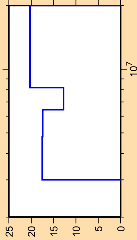
\Delta\sigma/\sigma vs. E for ^{149}\text{Ce}(n,2n)
