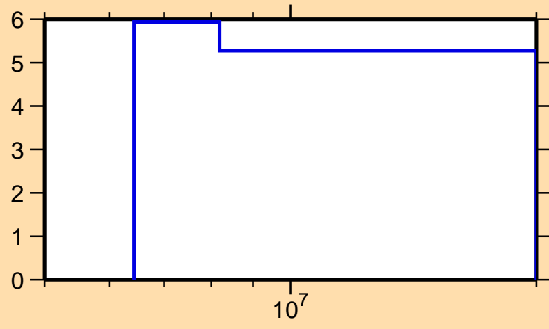
\Delta\sigma/\sigma vs. E for ^{149}\text{Ce}(n,\text{tot.})
