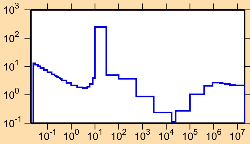
\sigma vs. E for ^{149}\text{Ce}(n,\text{nonel.})
