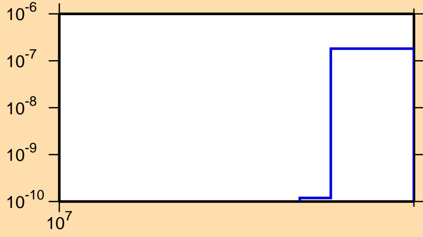
\sigma vs. E for ^{150}\text{Ce}(n,nt)
