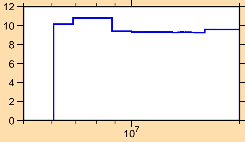
\Delta\sigma/\sigma vs. E for ^{150}\text{Ce}(n,\text{nonel.})
