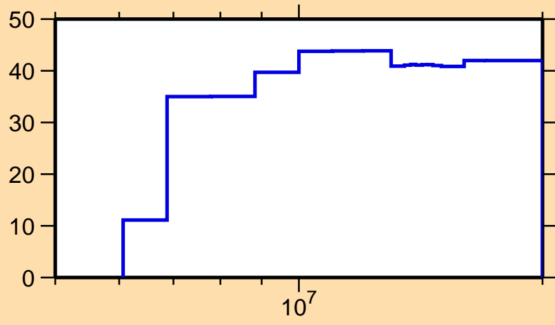
\Delta\sigma/\sigma vs. E for ^{150}\text{Ce}(n,\text{inel.})
