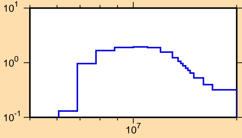
\sigma vs. E for ^{150}\text{Ce}(n,2n)
