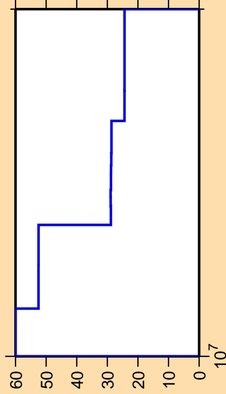
\Delta\sigma/\sigma vs. E for ^{150}\text{Ce}(n,3n)
