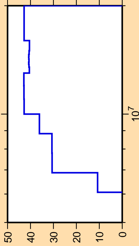
\Delta\sigma/\sigma vs. E for ^{150}\text{Ce}(n,n\text{cont.})
