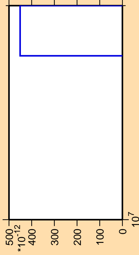
\Delta\sigma/\sigma vs. E for ^{150}\text{Ce} (mt 11)
