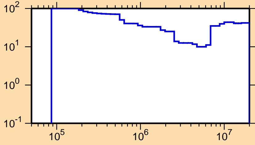
\Delta\sigma/\sigma vs. E for ^{150}\text{Ce}(n,\text{inel.})
