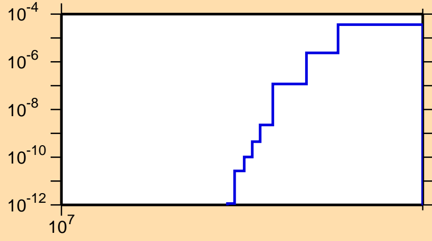
\sigma vs. E for ^{150}\text{Ce}(n,np)
