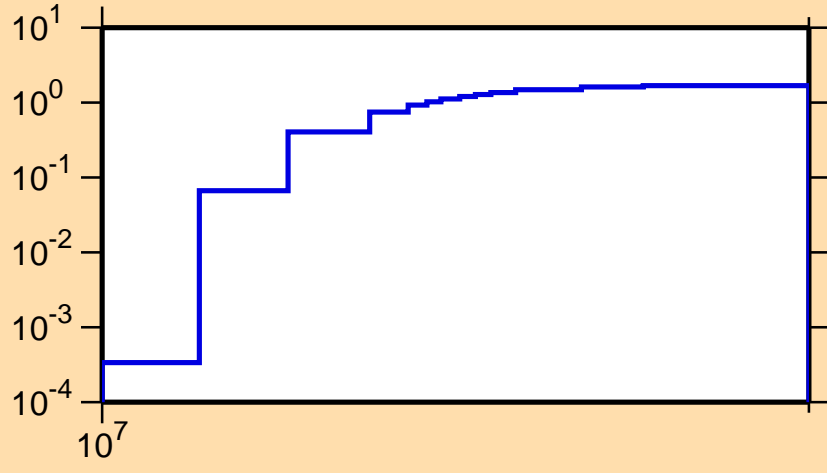
\sigma vs. E for ^{150}\text{Ce}(n,3n)
