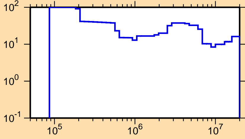
\Delta\sigma/\sigma vs. E for ^{150}\text{Ce}(n,\text{el.})
