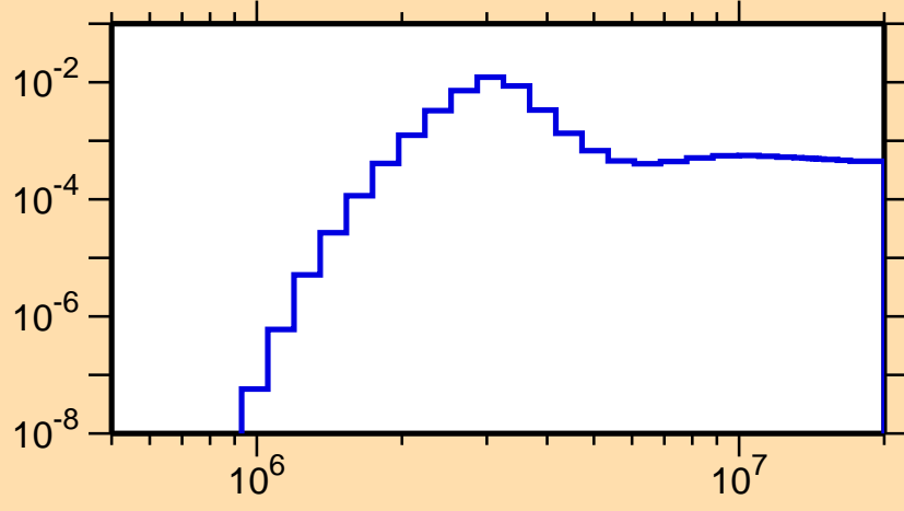
\sigma vs. E for ^{150}\text{Ce}(n,n_4)
