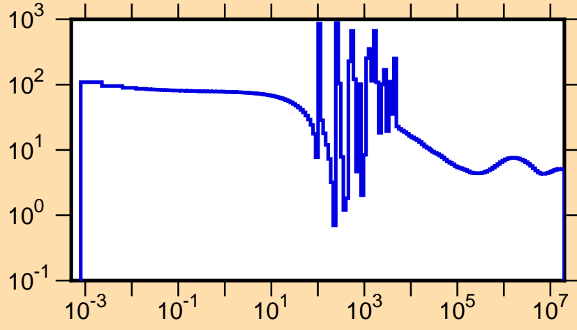
\sigma vs. E for ^{150}\text{Ce}(n,\text{tot.})
