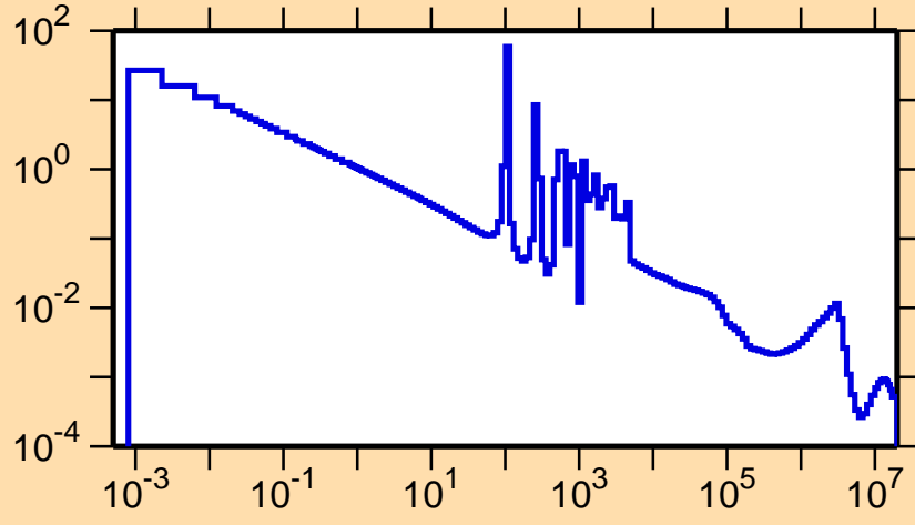
\sigma vs. E for ^{150}\text{Ce}(n,\gamma)
