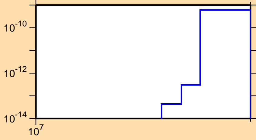
\sigma vs. E for ^{150}\text{Ce}(n,\text{nd})
