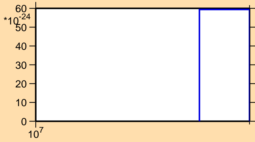
\sigma vs. E for ^{150}\text{Ce} (mt 11)
