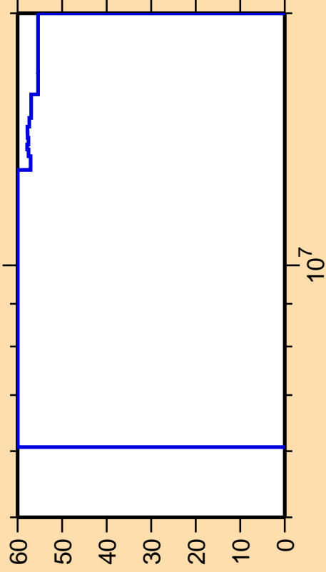
\Delta\sigma/\sigma vs. E for ^{150}\text{Ce}(n,n_1)
