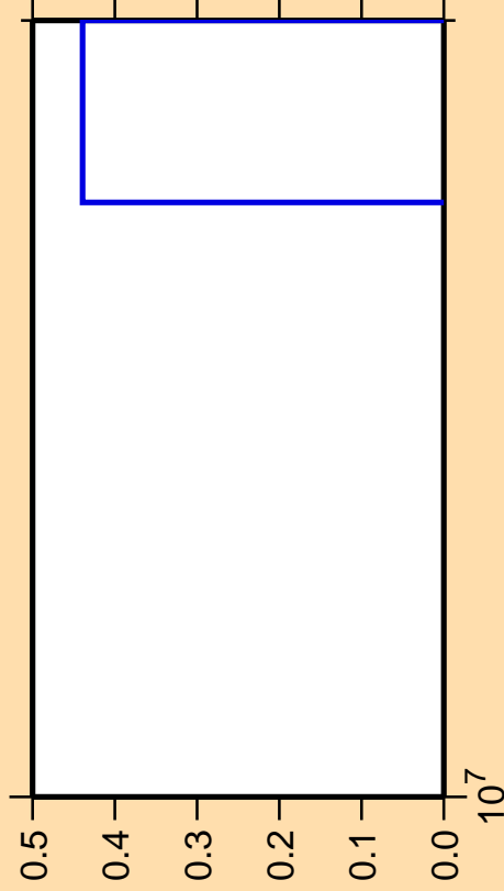
\Delta\sigma/\sigma vs. E for ^{150}\text{Ce}(n,2np)
