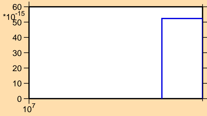
\sigma vs. E for ^{150}\text{Ce}(n,2np)
