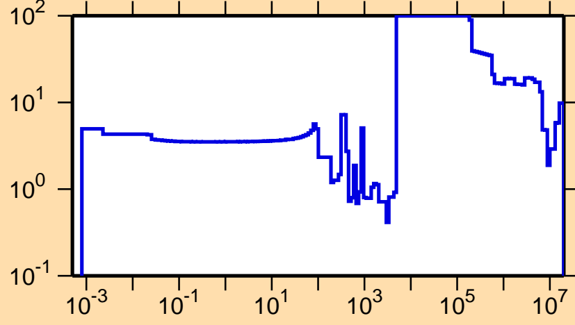
\Delta\sigma/\sigma vs. E for ^{150}\text{Ce}(n,\text{tot.})
