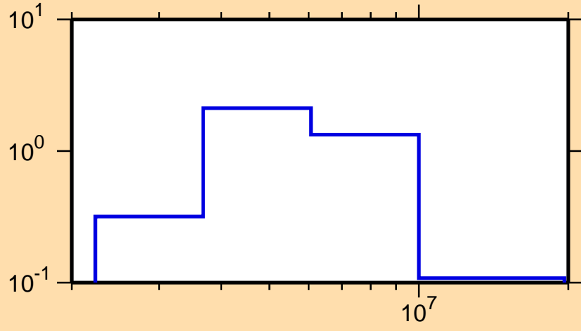
\sigma vs. E for ^{150}\text{Ce}(n,n\text{cont.})
