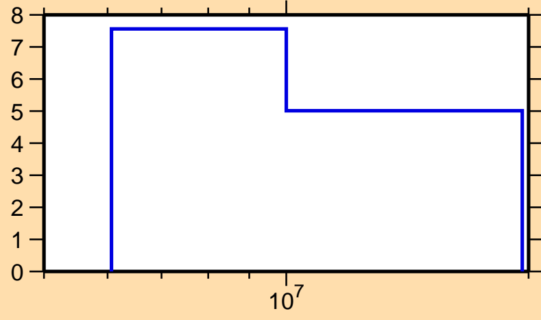
\Delta\sigma/\sigma vs. E for ^{150}\text{Ce}(n,\text{tot.})
