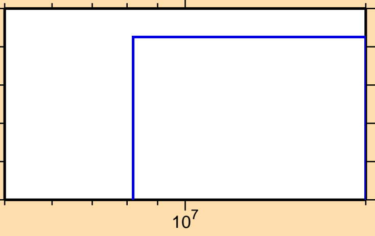
\sigma vs. E for ^{150}\text{Ce}(n,2np)
