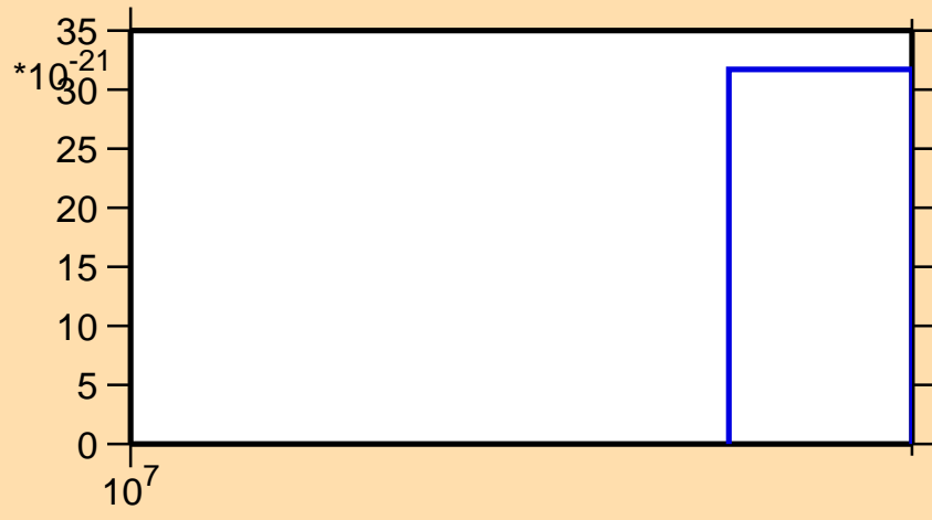
\sigma vs. E for ^{151}\text{Ce} (mt 11)
