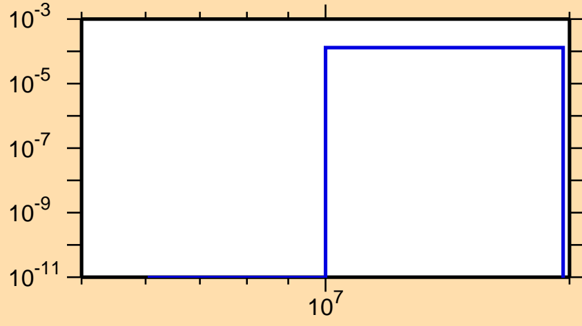
\sigma vs. E for ^{151}\text{Ce}(n,p)
