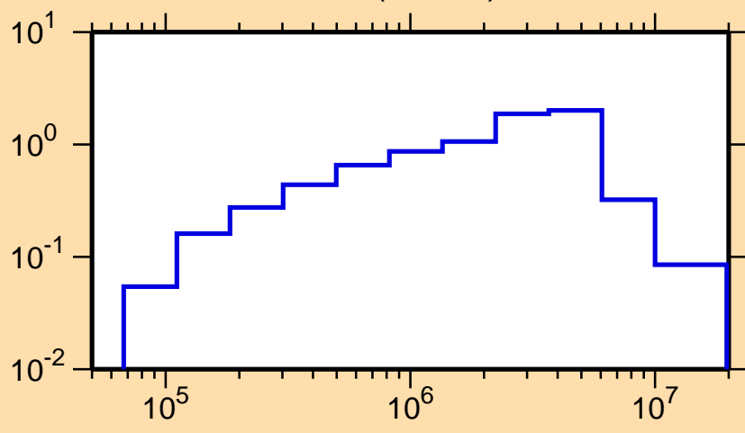
\sigma vs. E for ^{151}\text{Ce}(n,\text{inel.})
