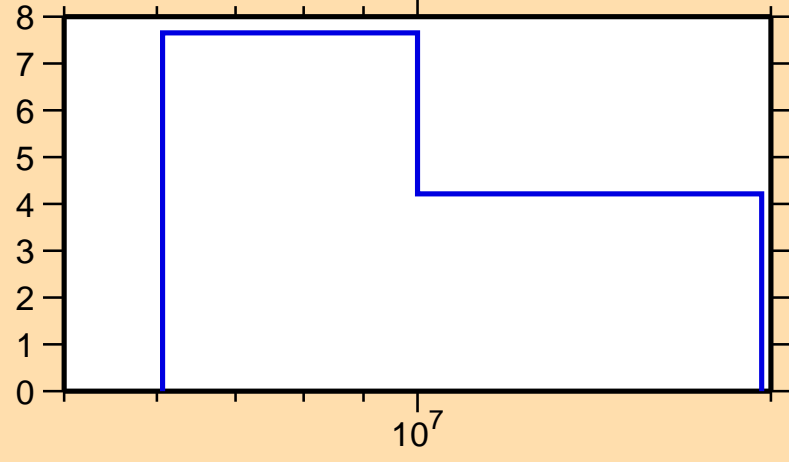
\Delta\sigma/\sigma vs. E for ^{151}\text{Ce}(n,\text{tot.})
