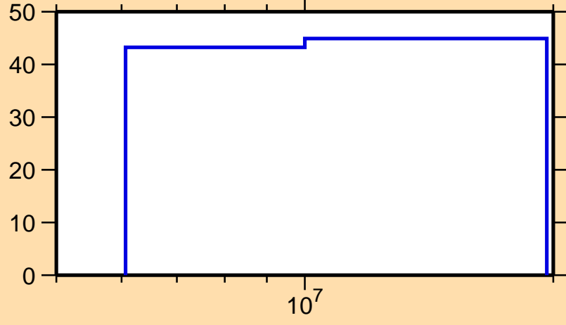
\Delta\sigma/\sigma vs. E for ^{151}\text{Ce}(n,n\text{cont.})
