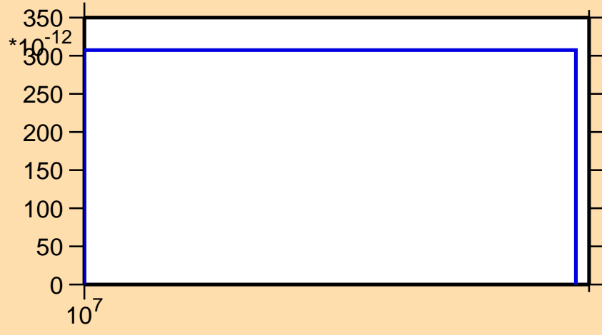
\sigma vs. E for ^{151}\text{Ce}(n,2n\alpha)
