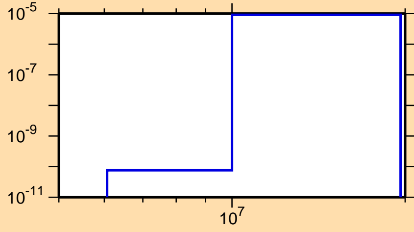
\sigma vs. E for ^{151}\text{Ce}(n,\alpha)
