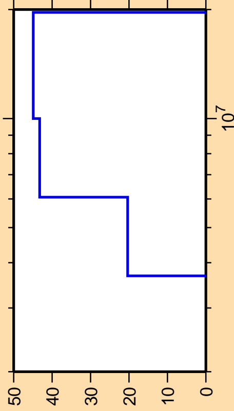
\Delta\sigma/\sigma vs. E for ^{151}\text{Ce}(n,n\text{cont.})
