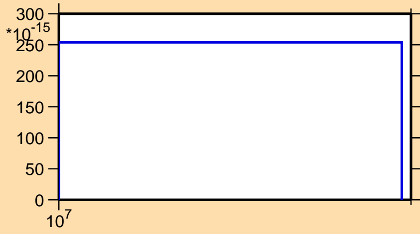
\sigma vs. E for ^{151}\text{Ce}(n,2np)
