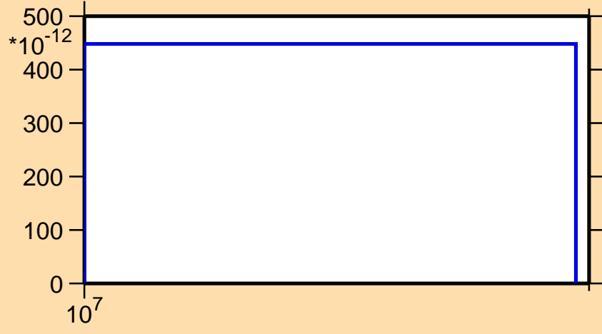
\sigma vs. E for ^{151}\text{Ce}(n,nt)
