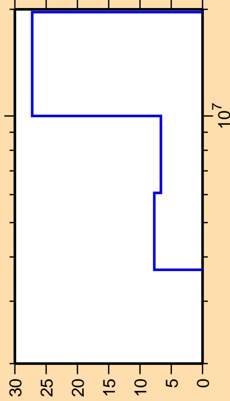
\Delta\sigma/\sigma vs. E for ^{151}\text{Ce}(n,2n)
