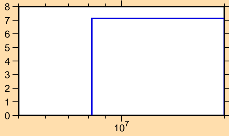
\Delta\sigma/\sigma vs. E for ^{151}\text{Ce}(n,\text{nonel.})
