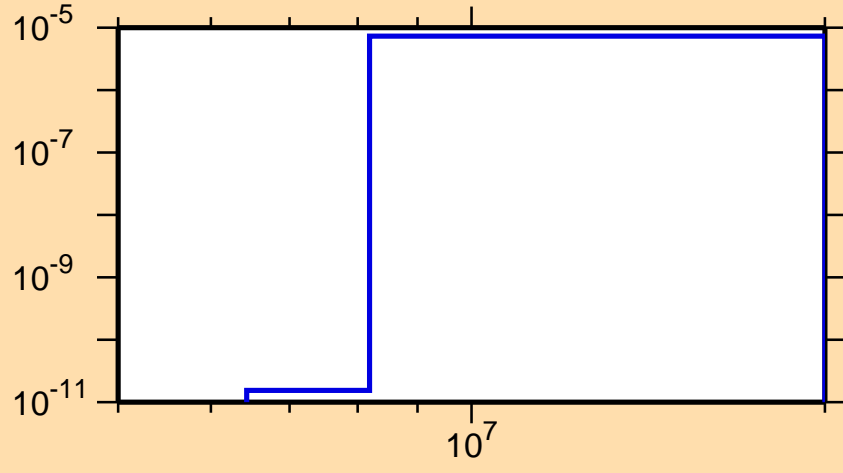
\sigma vs. E for ^{151}\text{Ce}(n,\alpha)
