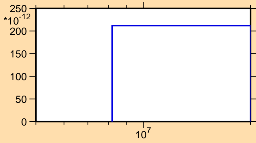
\sigma vs. E for ^{151}\text{Ce}(n,\text{nd})
