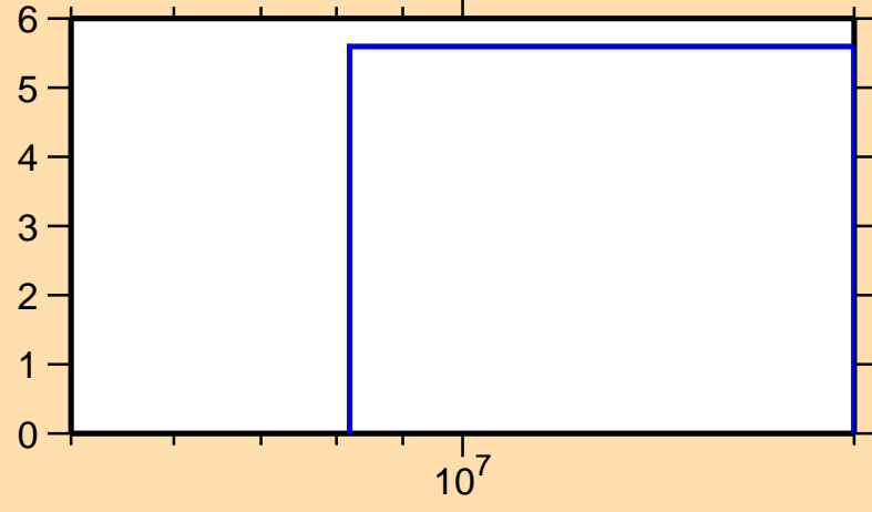
\Delta\sigma/\sigma vs. E for ^{151}\text{Ce}(n,\text{el.})
