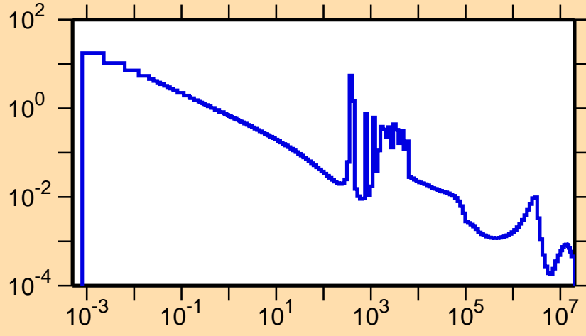
\sigma vs. E for ^{152}\text{Ce}(n,\gamma)
