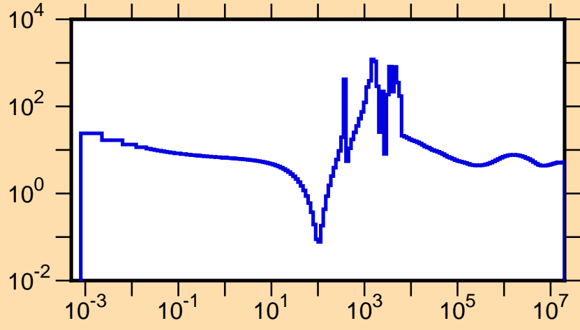
\sigma vs. E for ^{152}\text{Ce}(n,\text{tot.})
