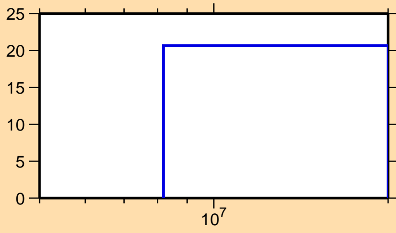
\Delta\sigma/\sigma vs. E for ^{152}\text{Ce}(n,n_1)
