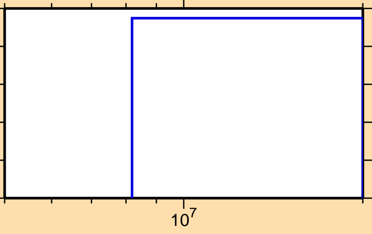
\sigma vs. E for ^{152}\text{Ce}(n,\text{nd})
