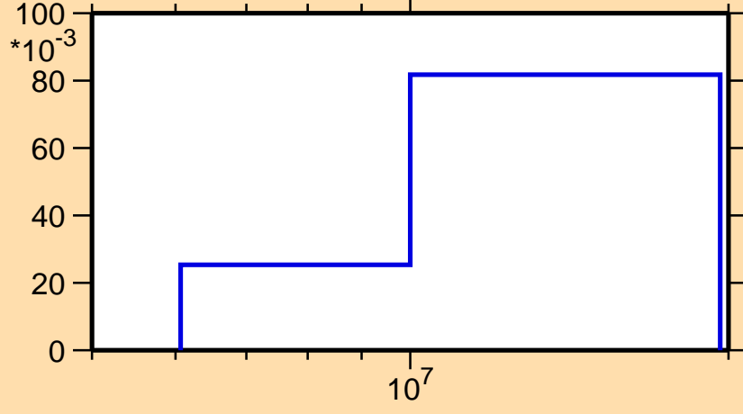
\sigma vs. E for ^{239}\text{Cf}(n,2n)
