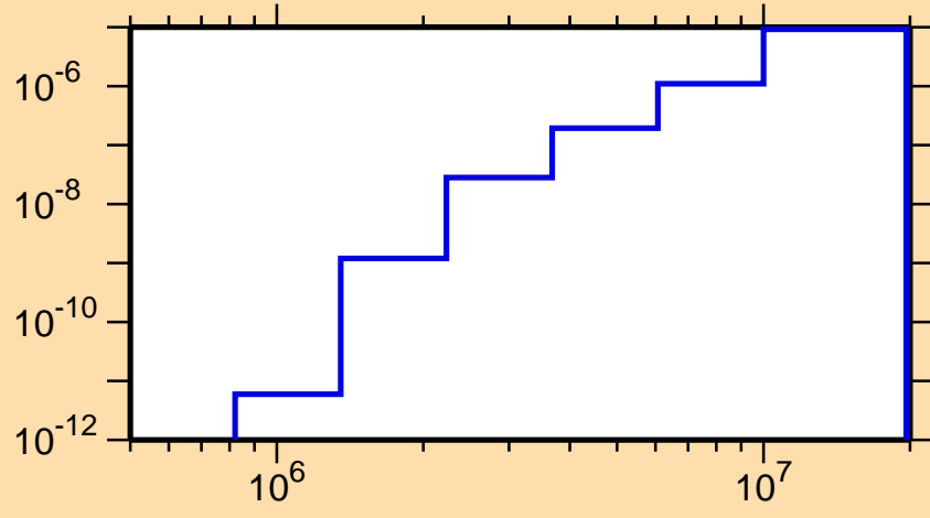
\sigma vs. E for ^{239}\text{Cf}(n,n\alpha)
