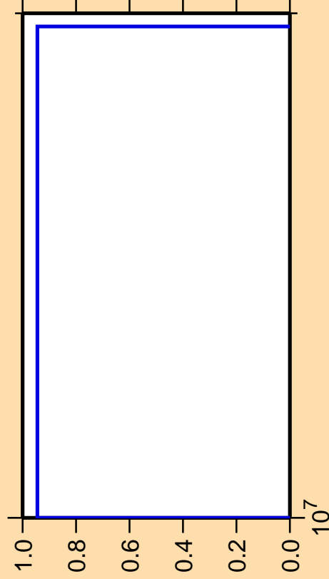
\Delta\sigma/\sigma vs. E for ^{239}\text{Cf} (mt 45)
