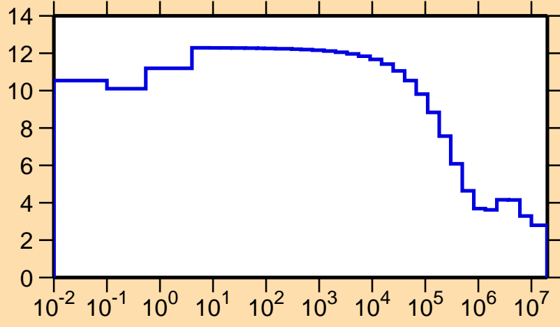
\sigma vs. E for ^{239}\text{Cf}(n,\text{el.})
