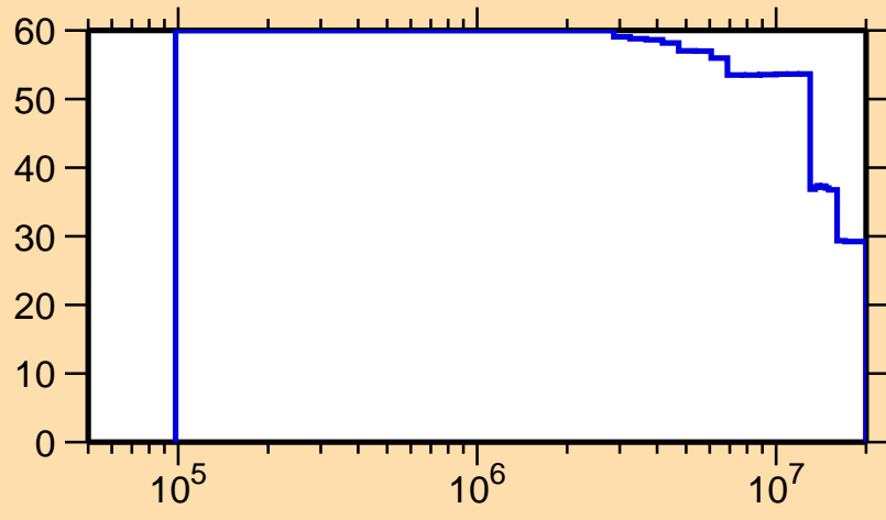
\Delta\sigma/\sigma vs. E for ^{240}\text{Cf}(n,f)
