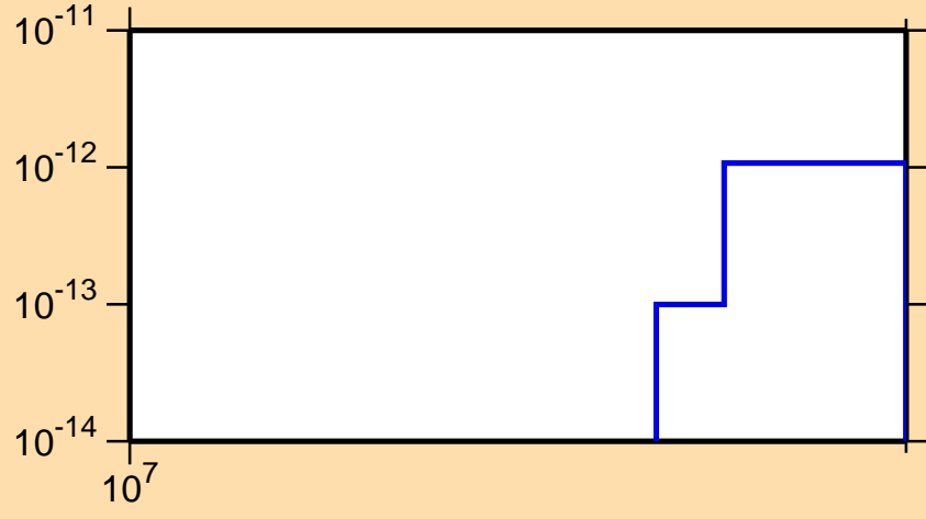
\sigma vs. E for ^{240}\text{Cf} (mt 45)
