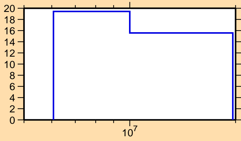
\Delta\sigma/\sigma vs. E for ^{240}\text{Cf}(n,\text{tot.})
