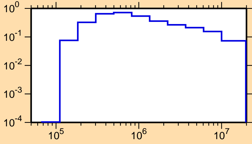
\sigma vs. E for ^{240}\text{Cf}(n,n_1)
