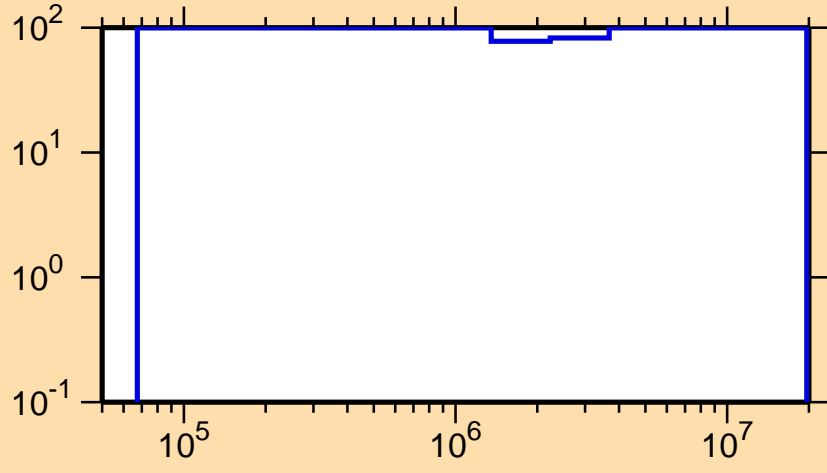
\Delta\sigma/\sigma vs. E for ^{240}\text{Cf}(n,n_1)
