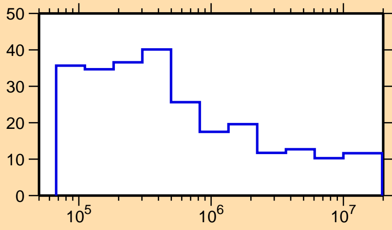
\Delta\sigma/\sigma vs. E for ^{240}\text{Cf}(n,\text{nonel.})
