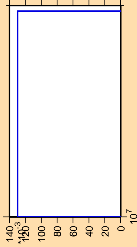
\Delta\sigma/\sigma vs. E for ^{240}\text{Cf} (mt 45)
