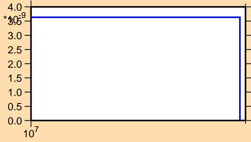
\sigma vs. E for ^{240}\text{Cf}(n,2np)
