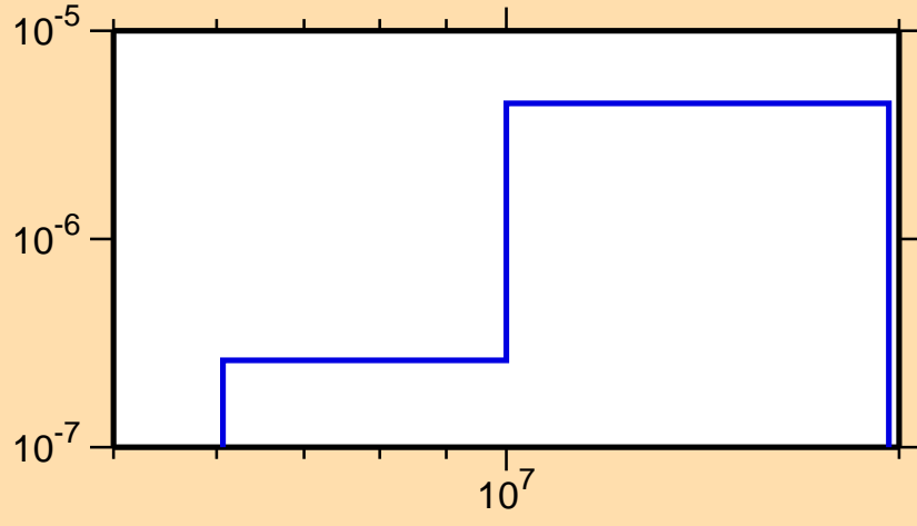
\sigma vs. E for ^{240}\text{Cf}(n,np)
