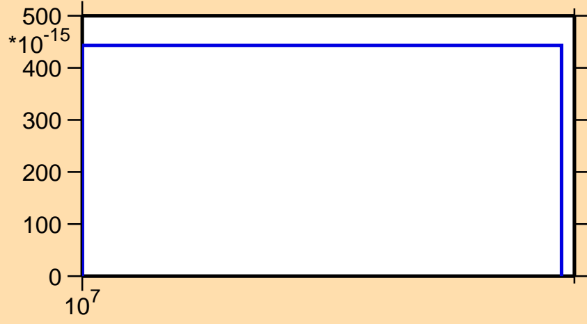
\sigma vs. E for ^{240}\text{Cf}(n,nd)
