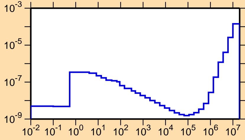
\sigma vs. E for ^{240}\text{Cf}(n,p)
