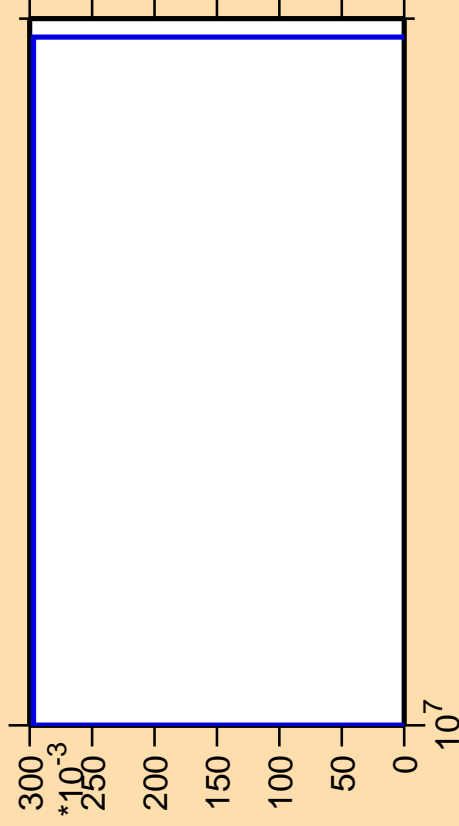
\Delta\sigma/\sigma vs. E for ^{240}\text{Cf}(n,nt)
