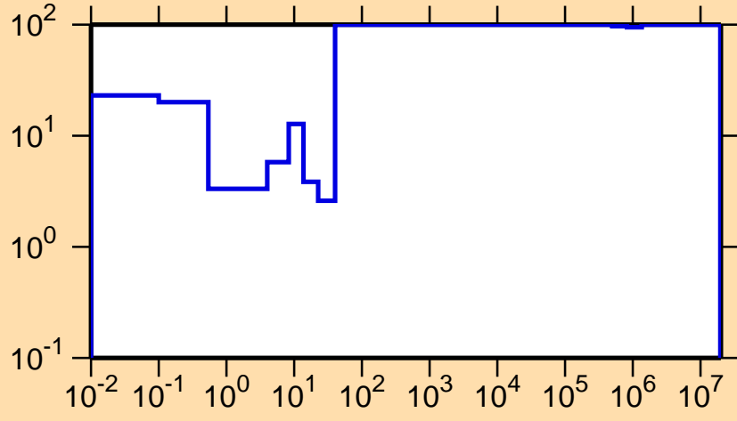
\Delta\sigma/\sigma vs. E for ^{240}\text{Cf}(n,\gamma)
