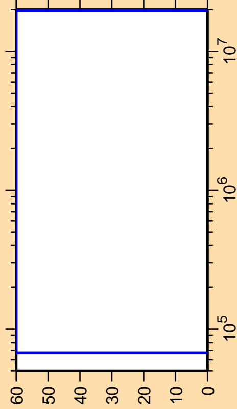
\Delta\sigma/\sigma vs. E for ^{240}\text{Cf}(n,\text{ncont.})
