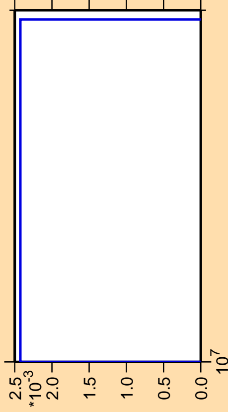
\Delta\sigma/\sigma vs. E for ^{240}\text{Cf}(\text{mt117})
