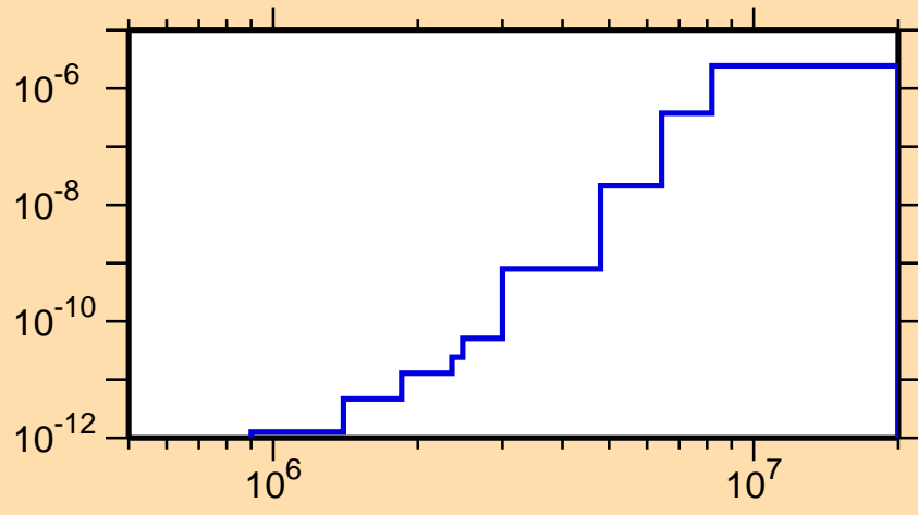
\sigma vs. E for ^{240}\text{Cf}(n,n\alpha)
