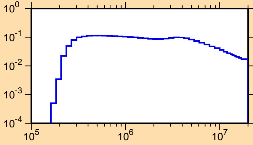
\sigma vs. E for ^{241}\text{Cf}(n,n_2)
