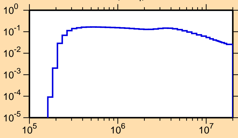
\sigma vs. E for ^{241}\text{Cf}(n,n_4)
