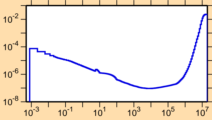
\sigma vs. E for ^{241}\text{Cf}(n,p)
