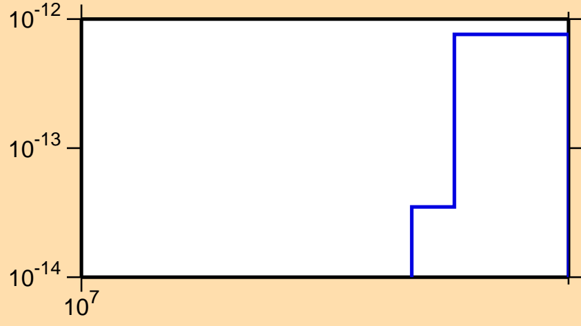
\sigma vs. E for ^{241}\text{Cf} (mt 45)
