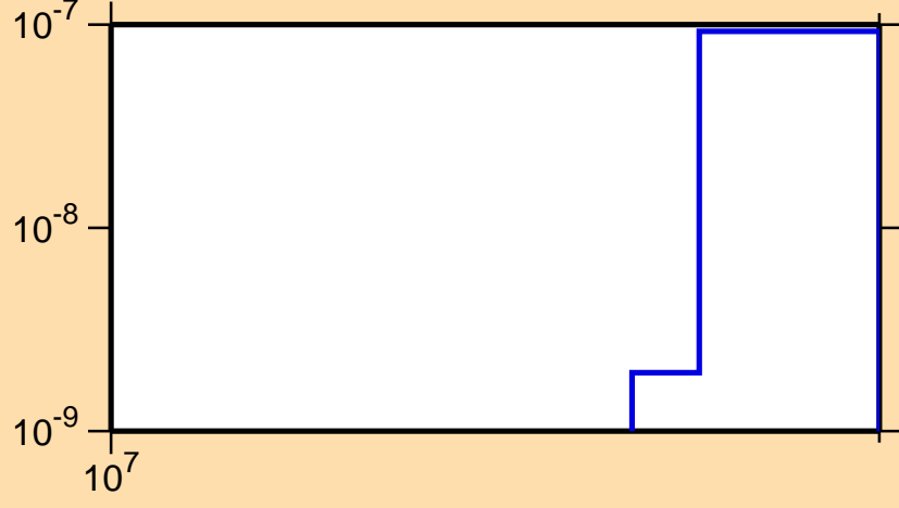
\sigma vs. E for ^{241}\text{Cf}(n,nt)
