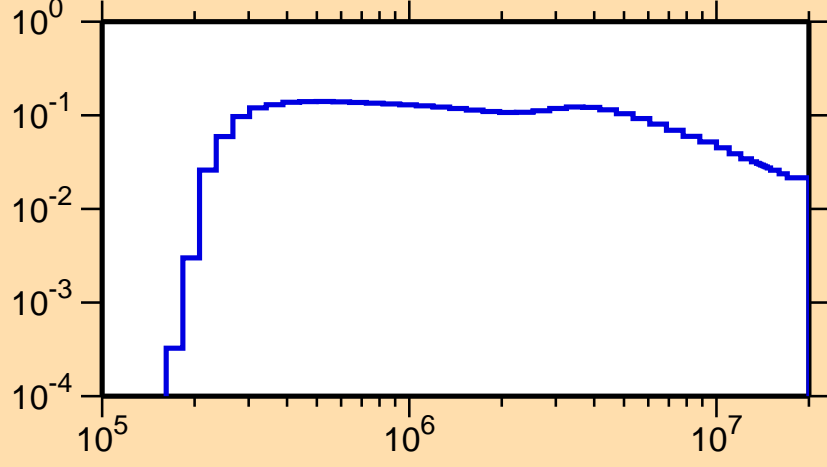
\sigma vs. E for ^{241}\text{Cf}(n,n_3)
