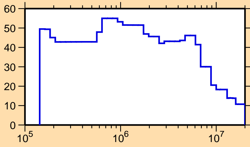
\Delta\sigma/\sigma vs. E for ^{241}\text{Cf}(n,f)
