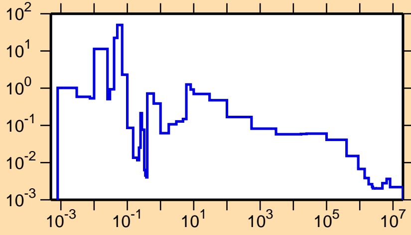
\sigma vs. E for ^{241}\text{Cf}(n,\gamma)
