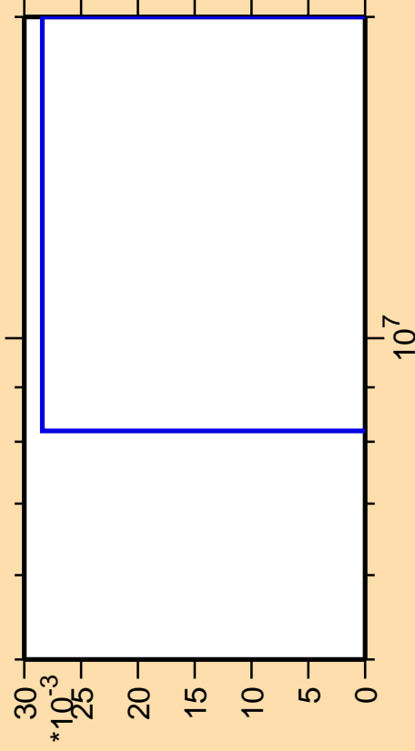
\Delta\sigma/\sigma vs. E for ^{241}\text{Cf}(\text{mt } 45)
