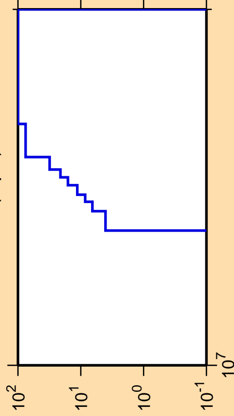
\Delta\sigma/\sigma vs. E for ^{242}\text{Cf}(n,p\alpha)
