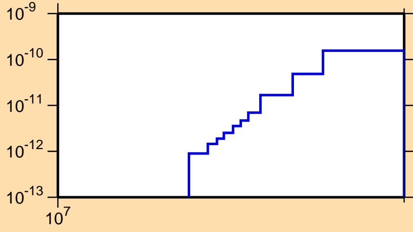
\sigma vs. E for ^{242}\text{Cf}(n,p\alpha)
