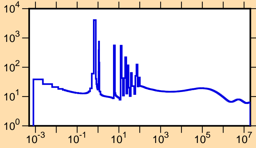
\sigma vs. E for ^{242}\text{Cf}(n,\text{tot.})
