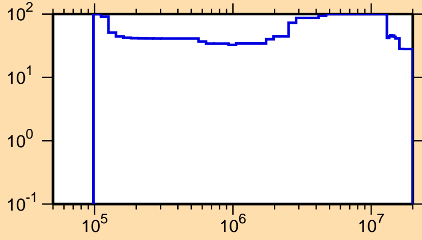
\Delta\sigma/\sigma vs. E for ^{242}\text{Cf}(n,\text{inel.})
