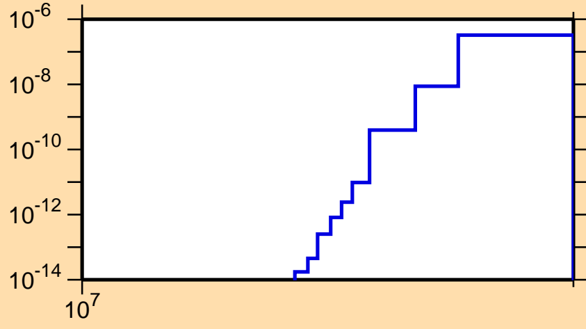
\sigma vs. E for ^{242}\text{Cf}(n,nd)
