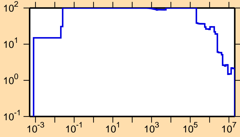
\Delta\sigma/\sigma vs. E for ^{242}\text{Cf}(n,\text{nonel.})
