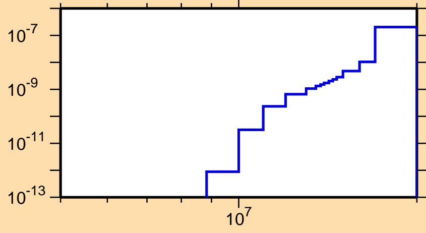
\sigma vs. E for ^{242}\text{Cf}(n,2n\alpha)
