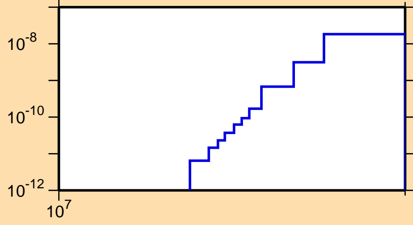
\sigma vs. E for ^{242}\text{Cf}(n,\text{He3})
