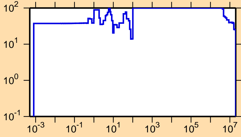
\Delta\sigma/\sigma vs. E for ^{242}\text{Cf}(n,f)
