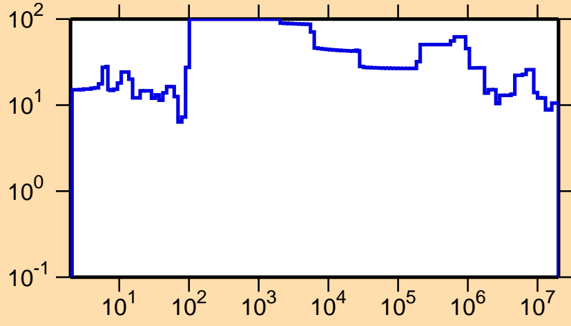
\Delta\sigma/\sigma vs. E for ^{242}\text{Cf}(n,\text{el.})
