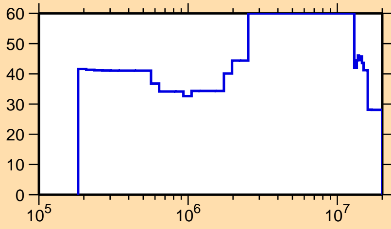
\Delta\sigma/\sigma vs. E for ^{242}\text{Cf}(n,\text{inel.})
