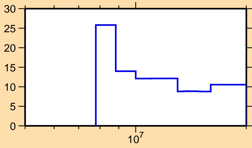
\Delta\sigma/\sigma vs. E for ^{242}\text{Cf}(n,\text{el.})
