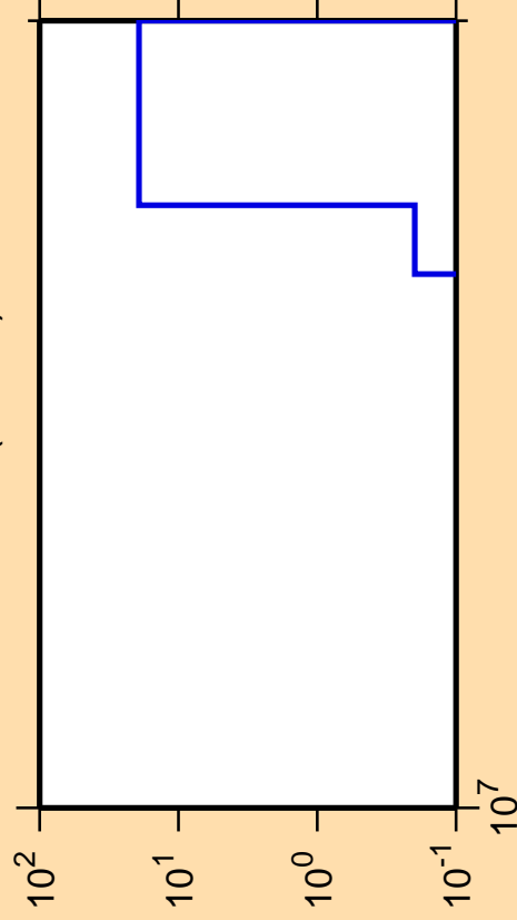
\Delta\sigma/\sigma vs. E for ^{242}\text{Cf}(\text{mt } 34)
