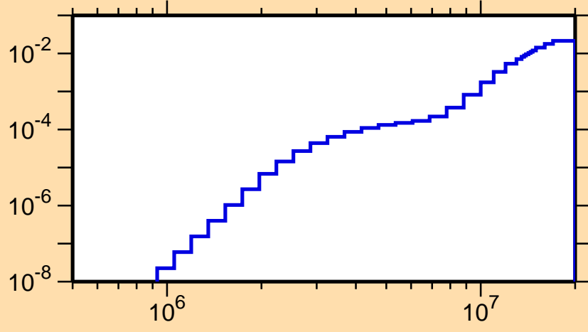
\sigma vs. E for ^{242}\text{Cf}(n,p)
