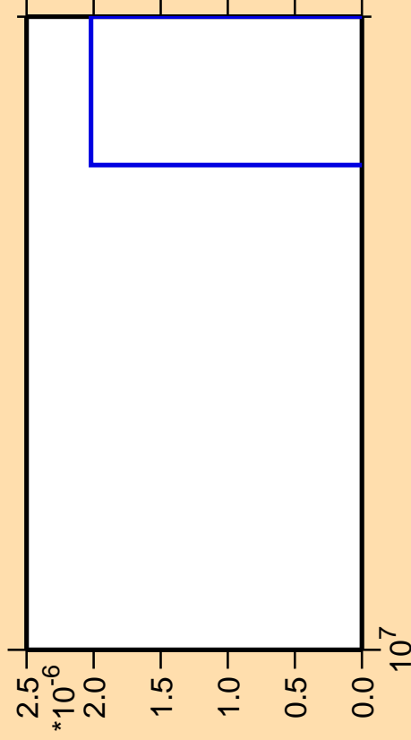
\Delta\sigma/\sigma vs. E for ^{242}\text{Cf}(\text{mt } 42)
