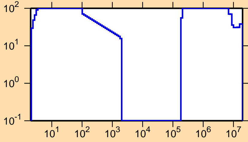
\Delta\sigma/\sigma vs. E for ^{242}\text{Cf}(n,p)
