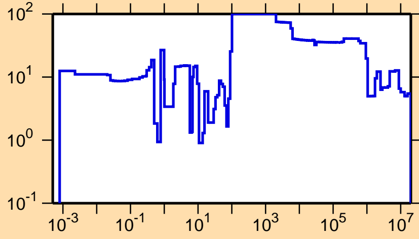
\Delta\sigma/\sigma vs. E for ^{242}\text{Cf}(n,\text{tot.})
