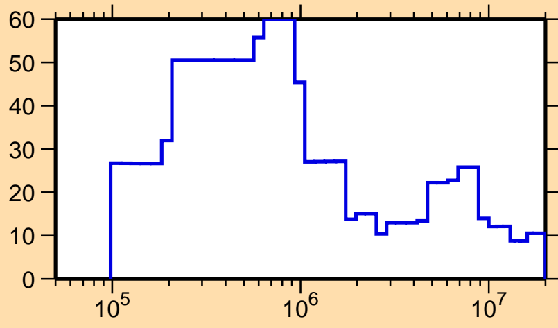
\Delta\sigma/\sigma vs. E for ^{242}\text{Cf}(n,el.)
