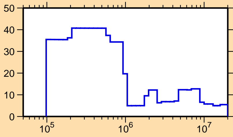
\Delta\sigma/\sigma vs. E for ^{242}\text{Cf}(n,\text{tot.})
