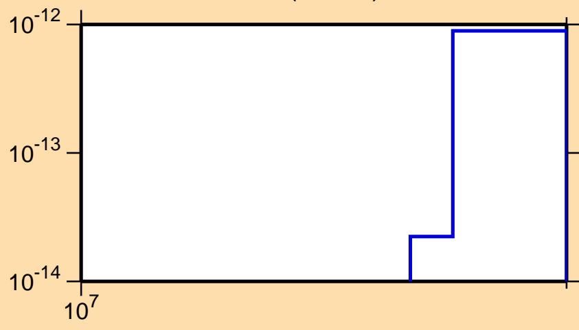
\sigma vs. E for ^{242}\text{Cf}(n,3n\alpha)
