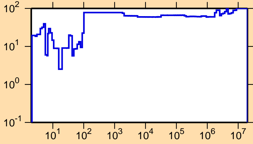
\Delta\sigma/\sigma vs. E for ^{242}\text{Cf}(n,\gamma)
