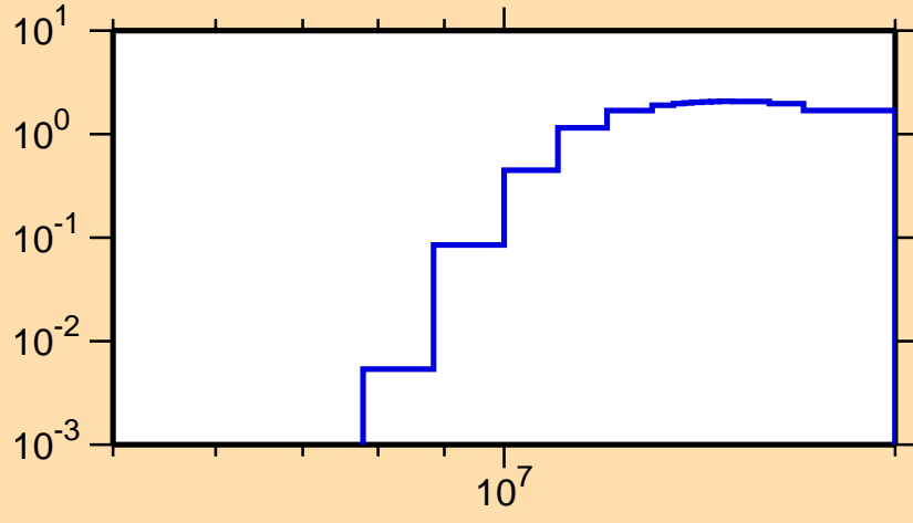
\sigma vs. E for ^{242}\text{Cf}(n,2n)
