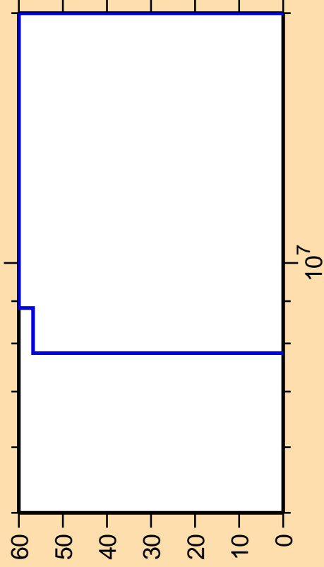
\Delta\sigma/\sigma vs. E for ^{242}\text{Cf}(n,n_1)
