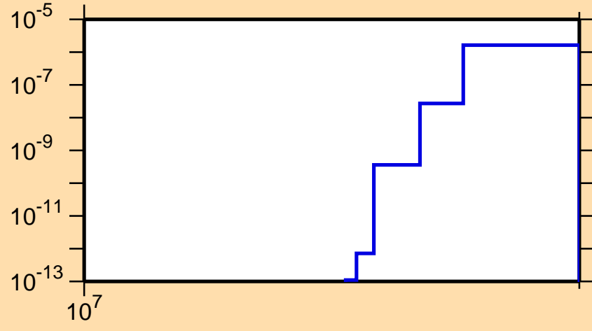
\sigma vs. E for ^{242}\text{Cf}(n,2np)
