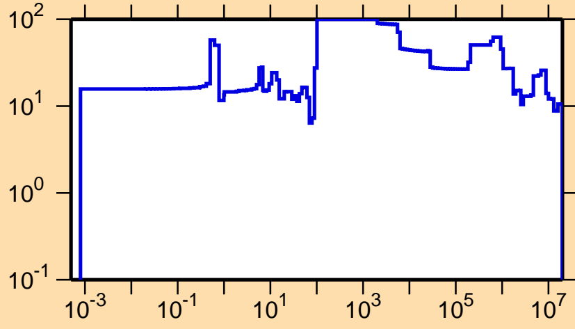
\Delta\sigma/\sigma vs. E for ^{242}\text{Cf}(n,el.)
