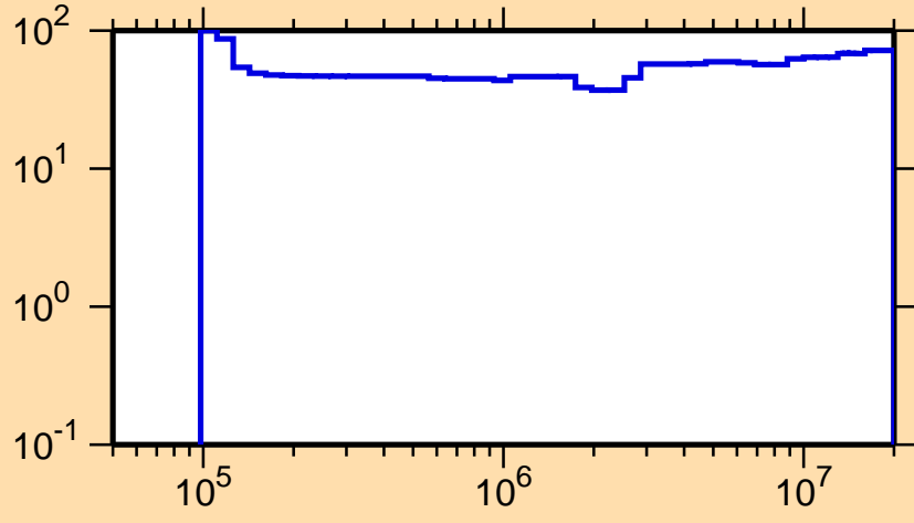
\Delta\sigma/\sigma vs. E for ^{242}\text{Cf}(n,n_1)
