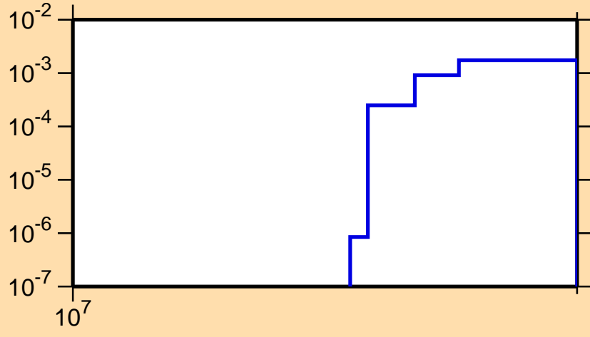
\sigma vs. E for ^{242}\text{Cf}(n,3n)
